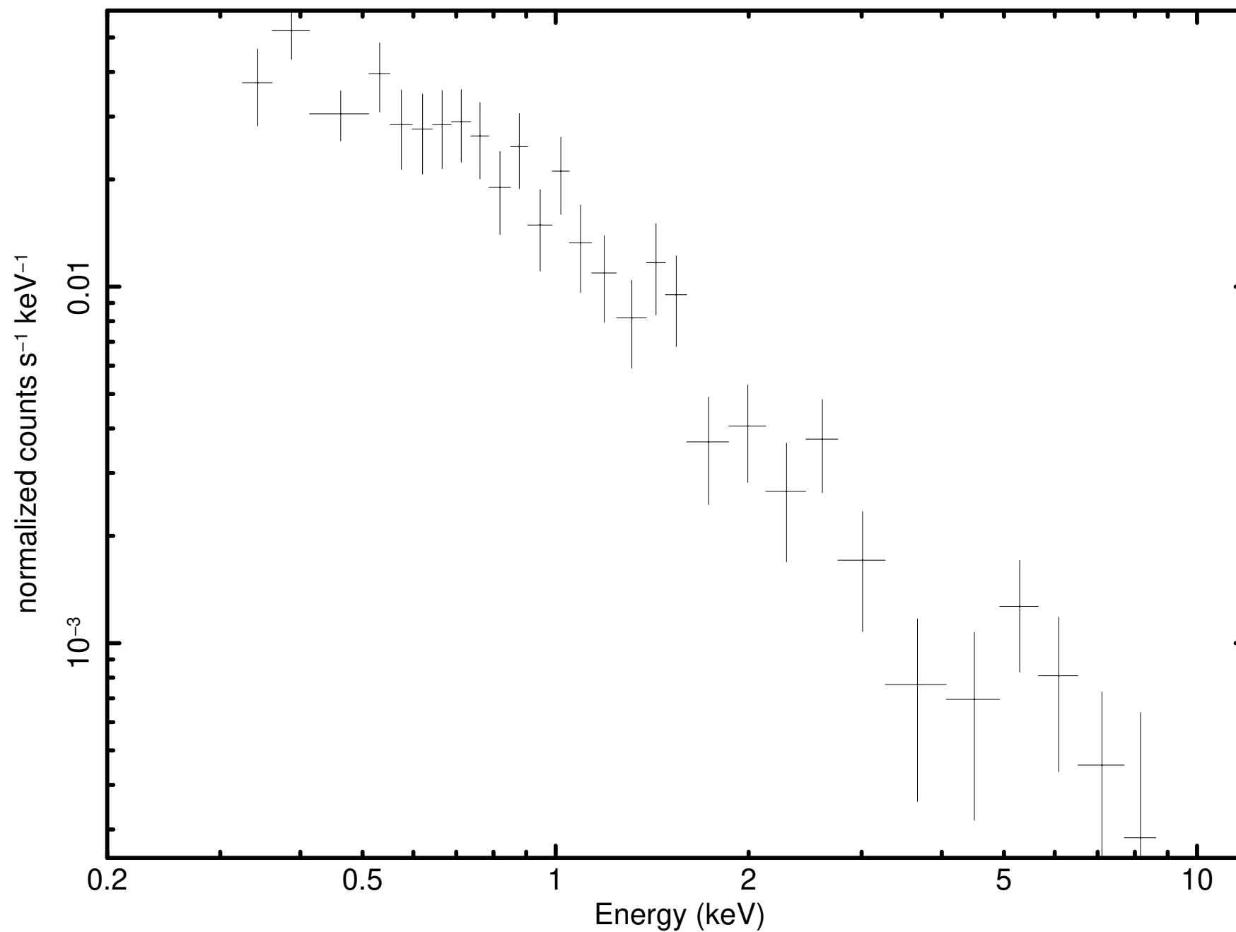
Source 8 minus background (P0921180301PNS003SRSPEC0008)
