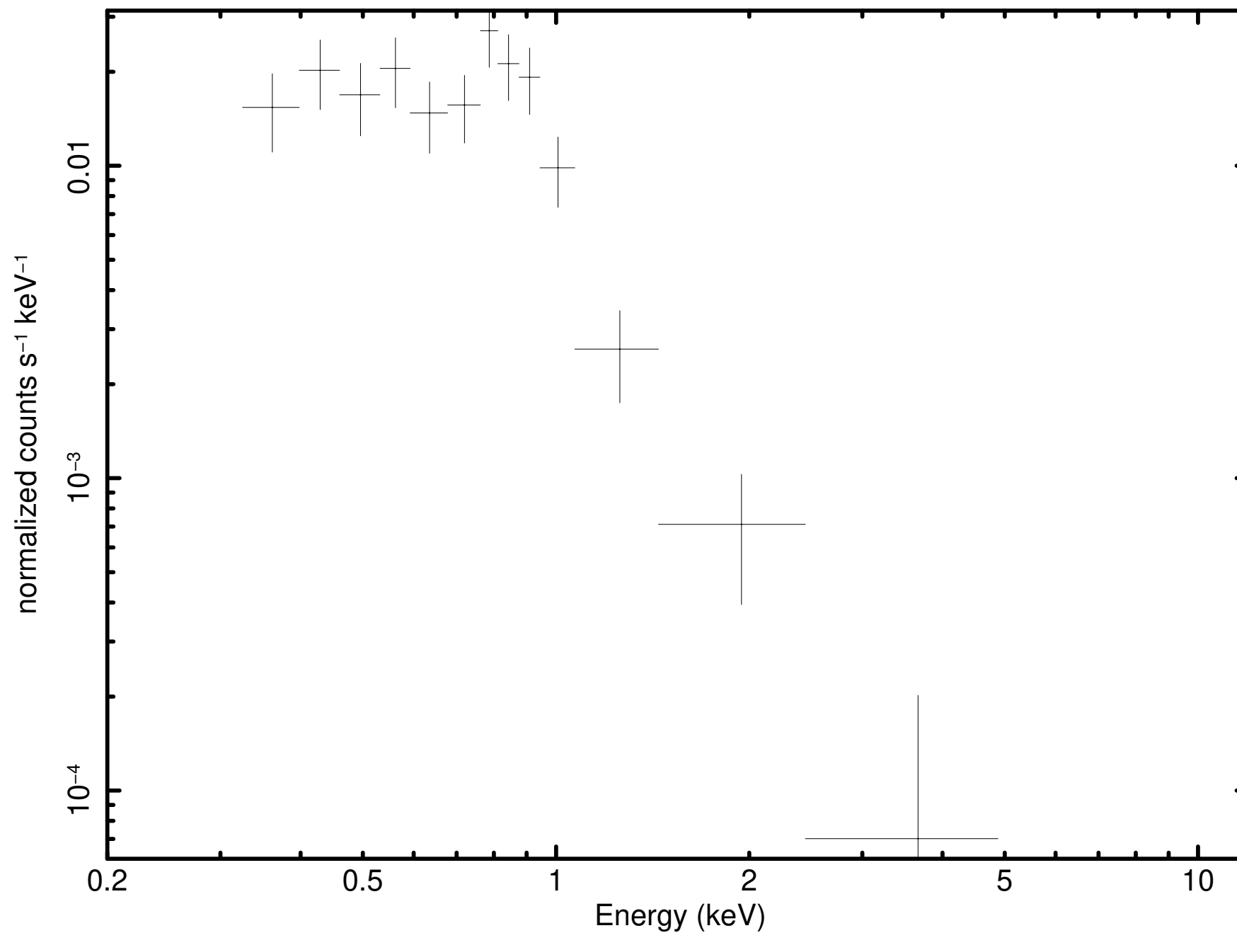
Source 9 minus background (P0921180301PNS003SRSPEC0009)
