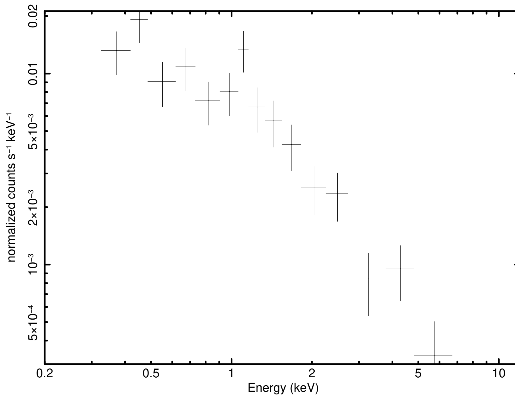
Source 10 minus background (P0921180301PNS003SRSPEC000A)
