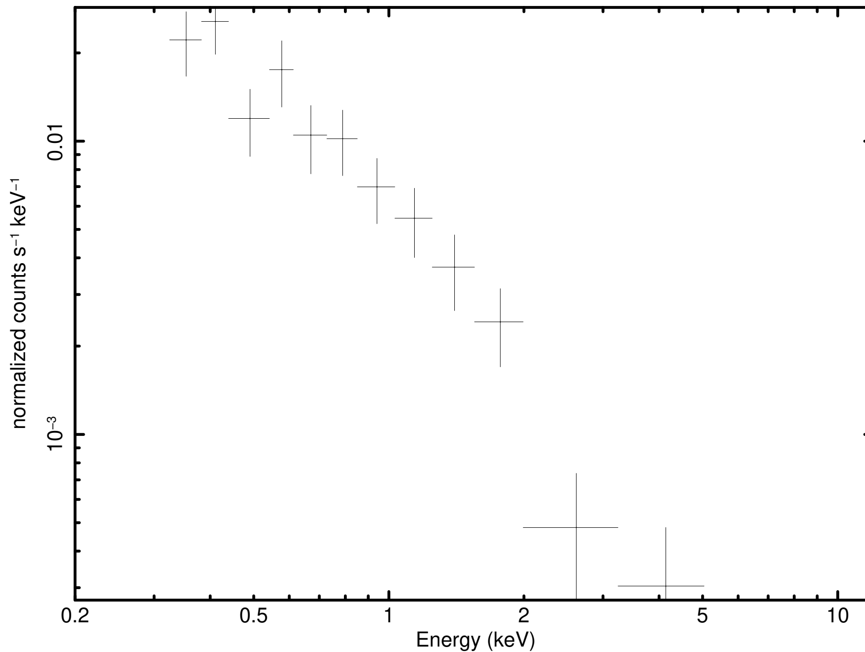
Source 11 minus background (P0921180301PNS003SRSPEC000B)
