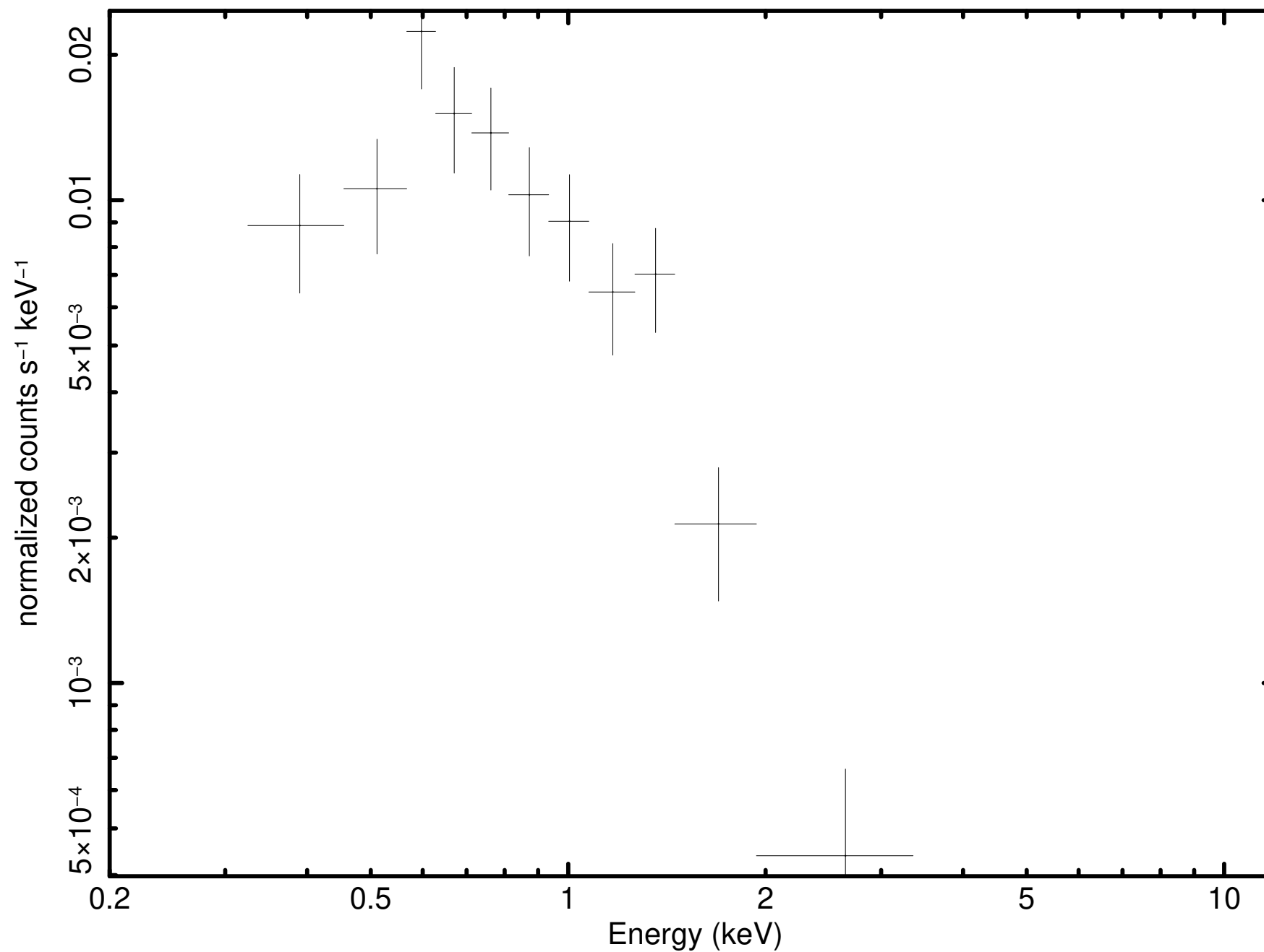
Source 12 minus background (P0921180301PNS003SRSPEC000C)
