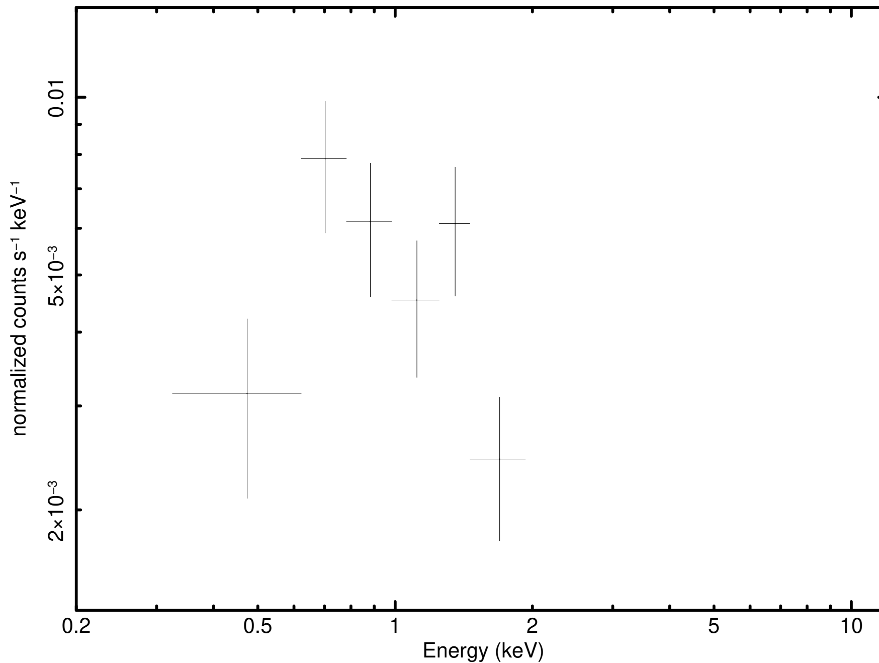
Source 13 minus background (P0921180301PNS003SRSPEC000D)
