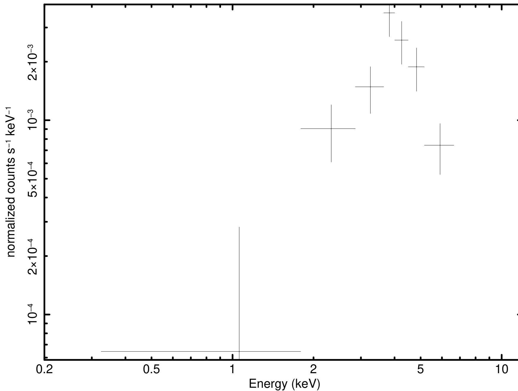
Source 16 minus background (P0921180301PNS003SRSPEC0010)
