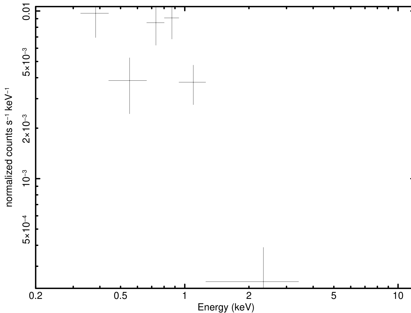
Source 17 minus background (P0921180301PNS003SRSPEC0011)
