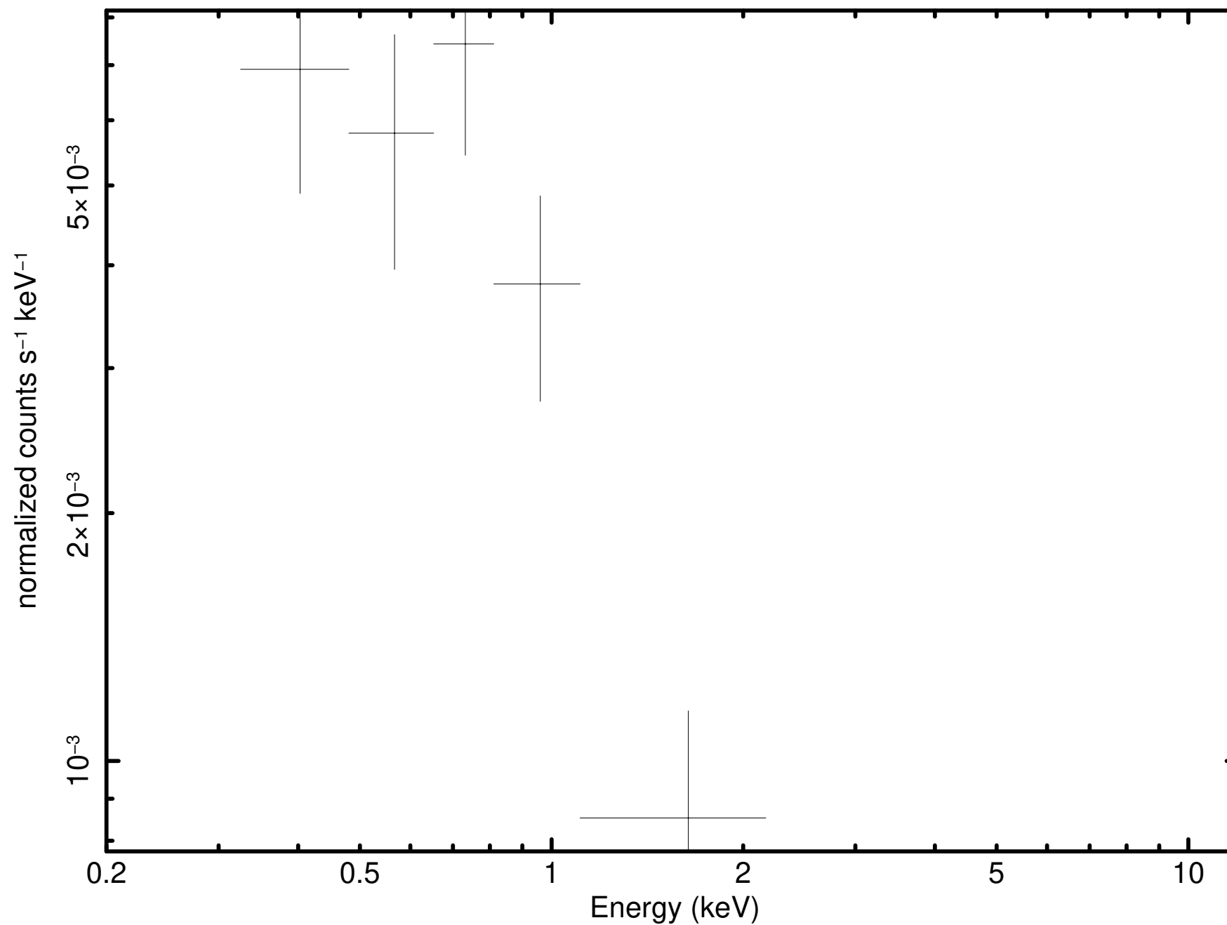
Source 18 minus background (P0921180301PNS003SRSPEC0012)
