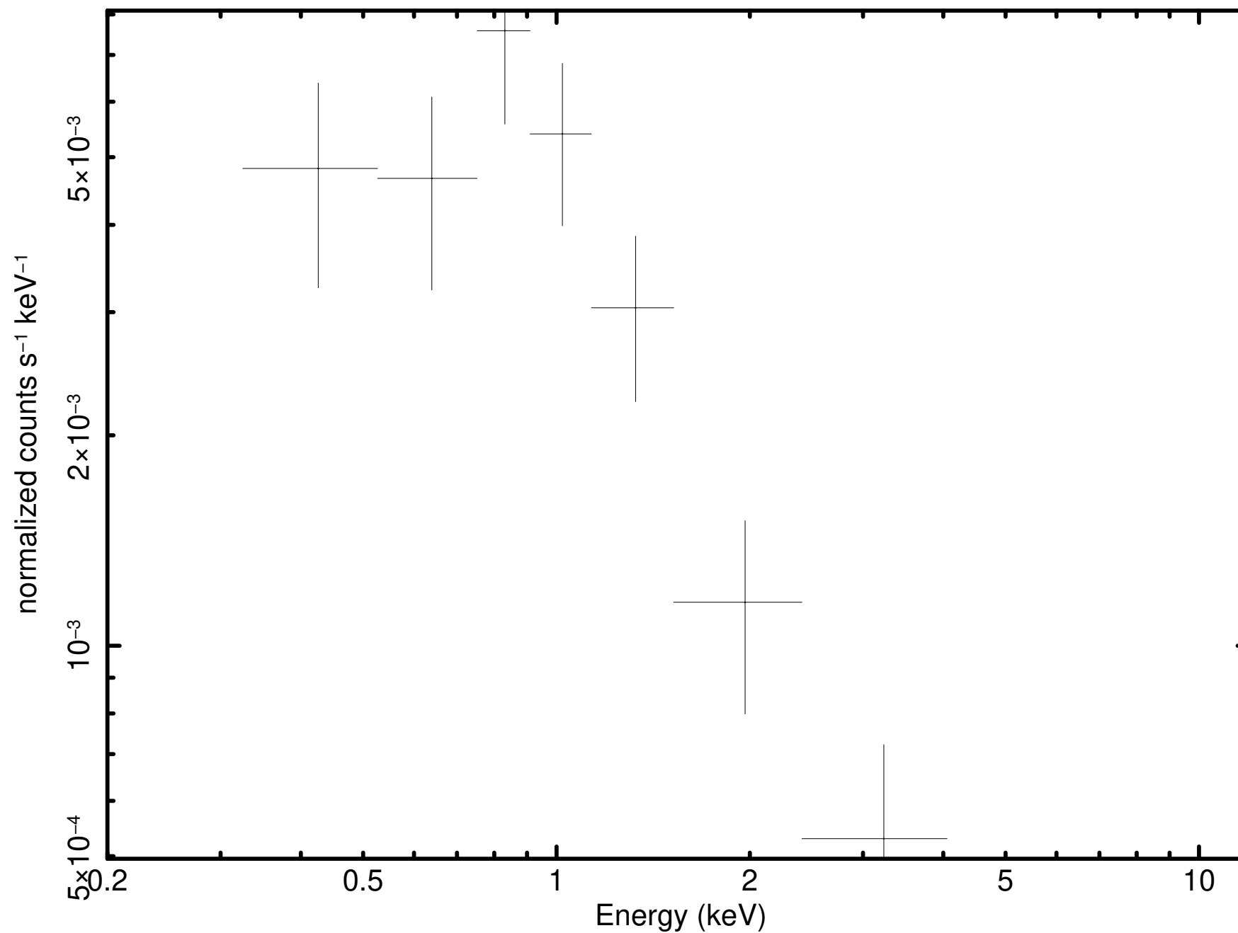
Source 19 minus background (P0921180301PNS003SRSPEC0013)
