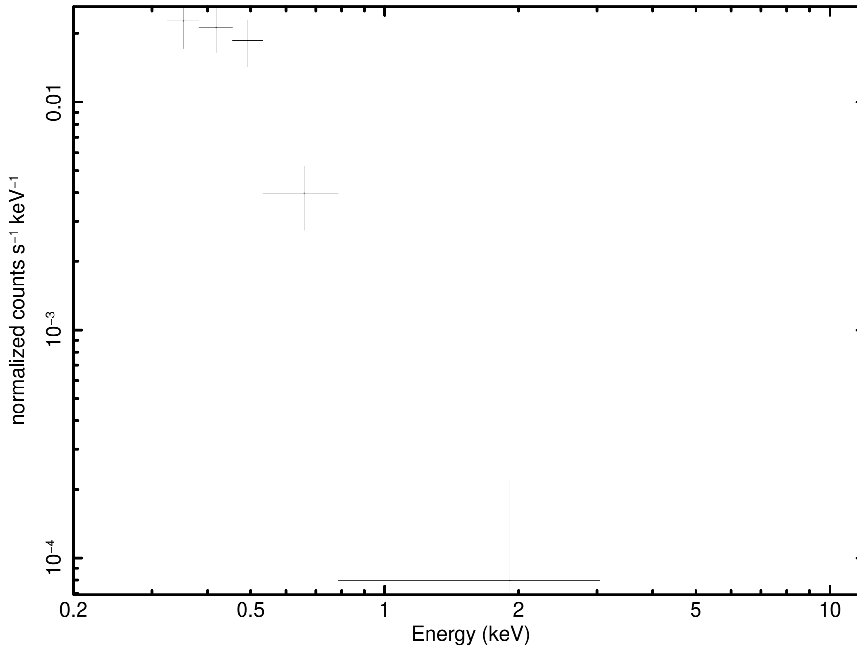
Source 21 minus background (P0921180301PNS003SRSPEC0015)
