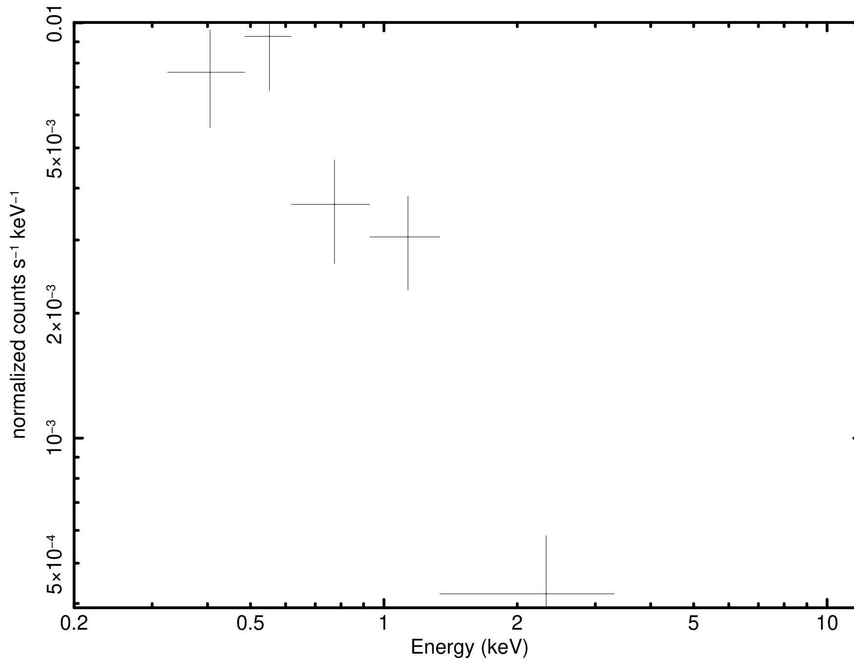
Source 23 minus background (P0921180301PNS003SRSPEC0017)
