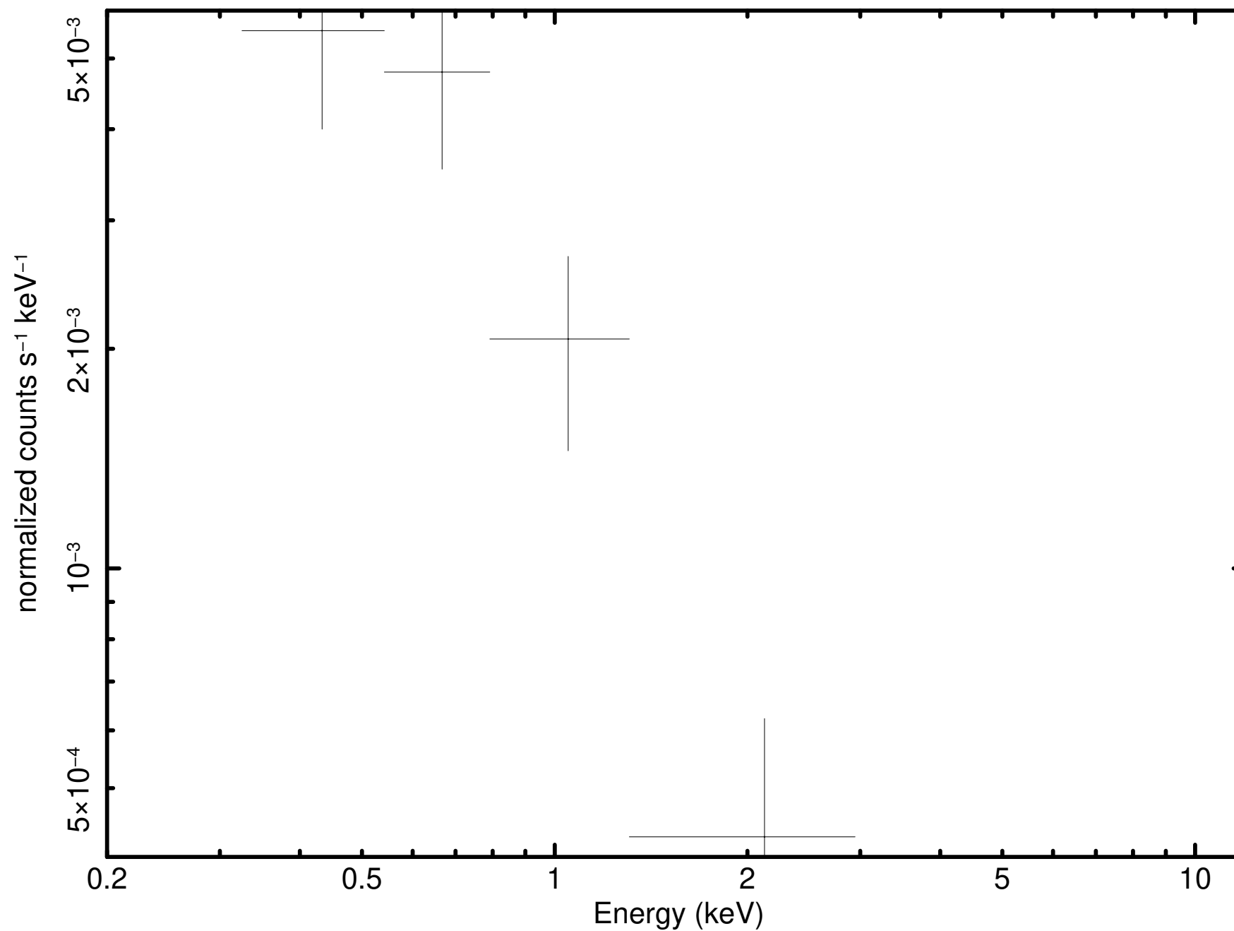
Source 33 minus background (P0921180301PNS003SRSPEC0021)
