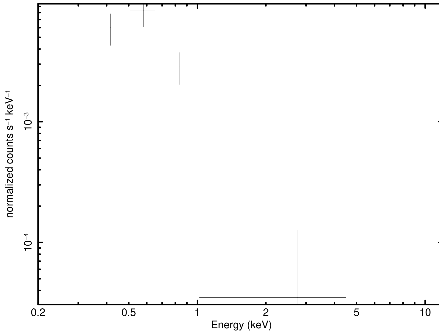
Source 46 minus background (P0921180301PNS003SRSPEC002E)
