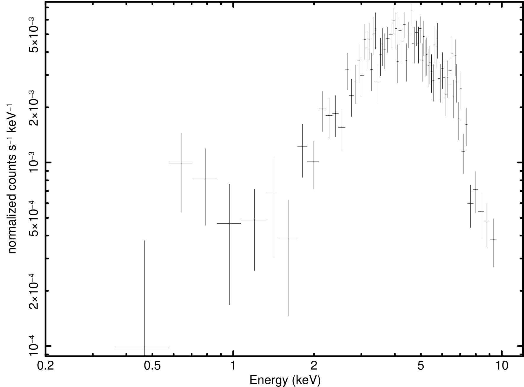
Source 1 minus background (P0931790101M1S001SRSPEC0001)
