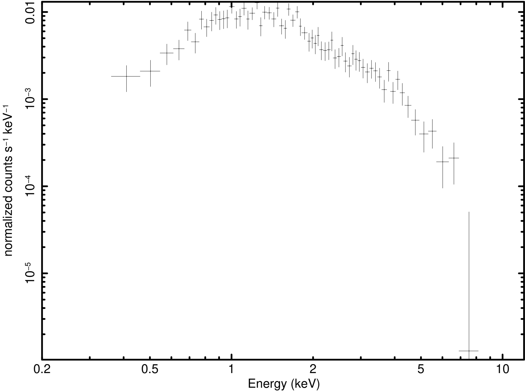
Source 2 minus background (P0931790101M1S001SRSPEC0002)
