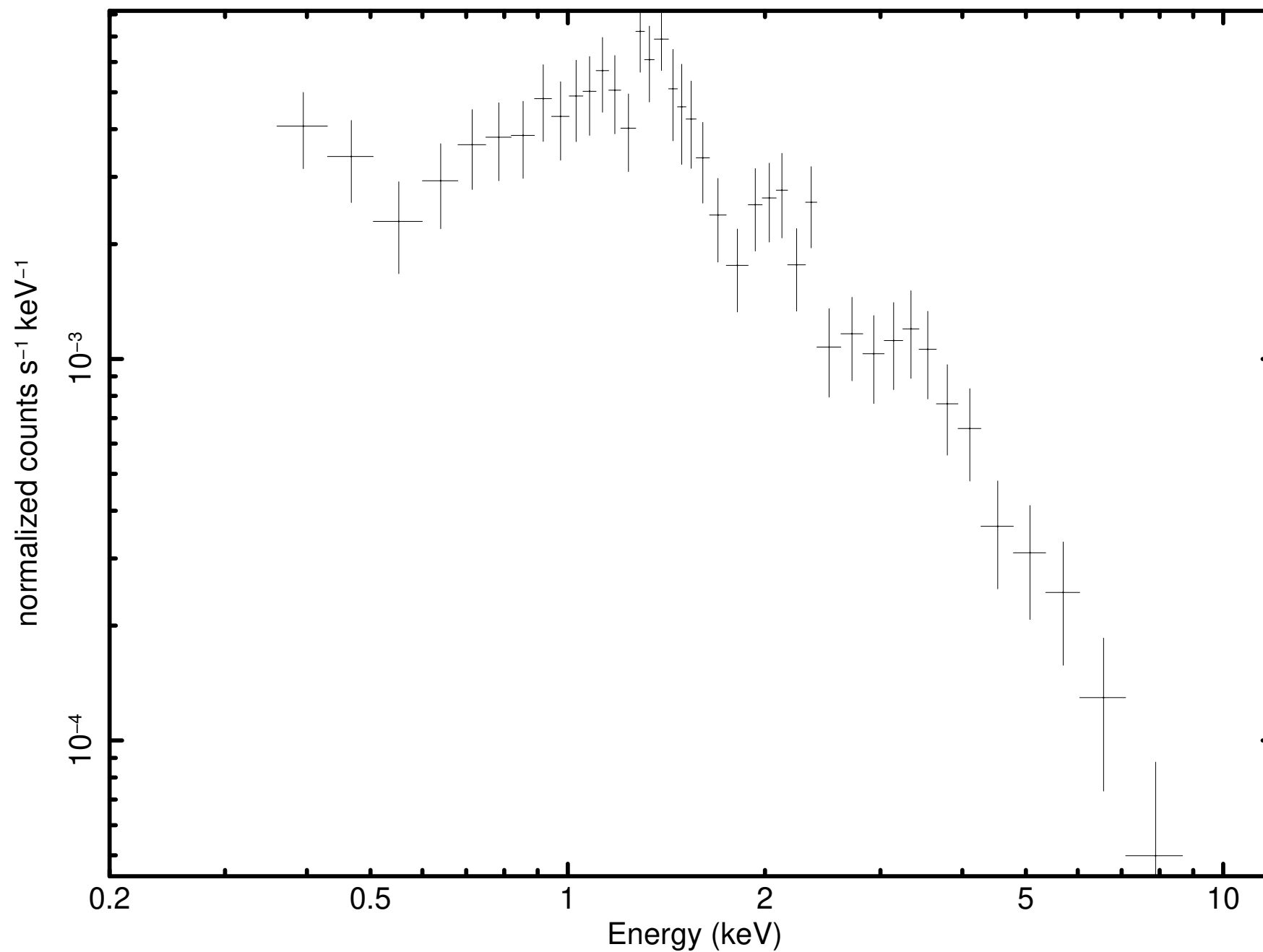
Source 4 minus background (P0931790101M1S001SRSPEC0004)
