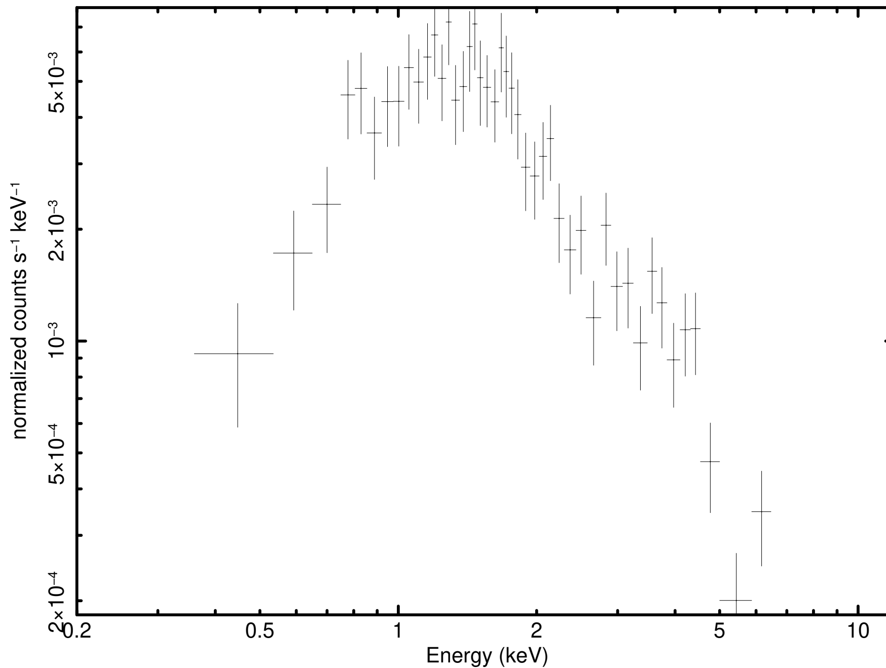
Source 5 minus background (P0931790101M1S001SRSPEC0005)
