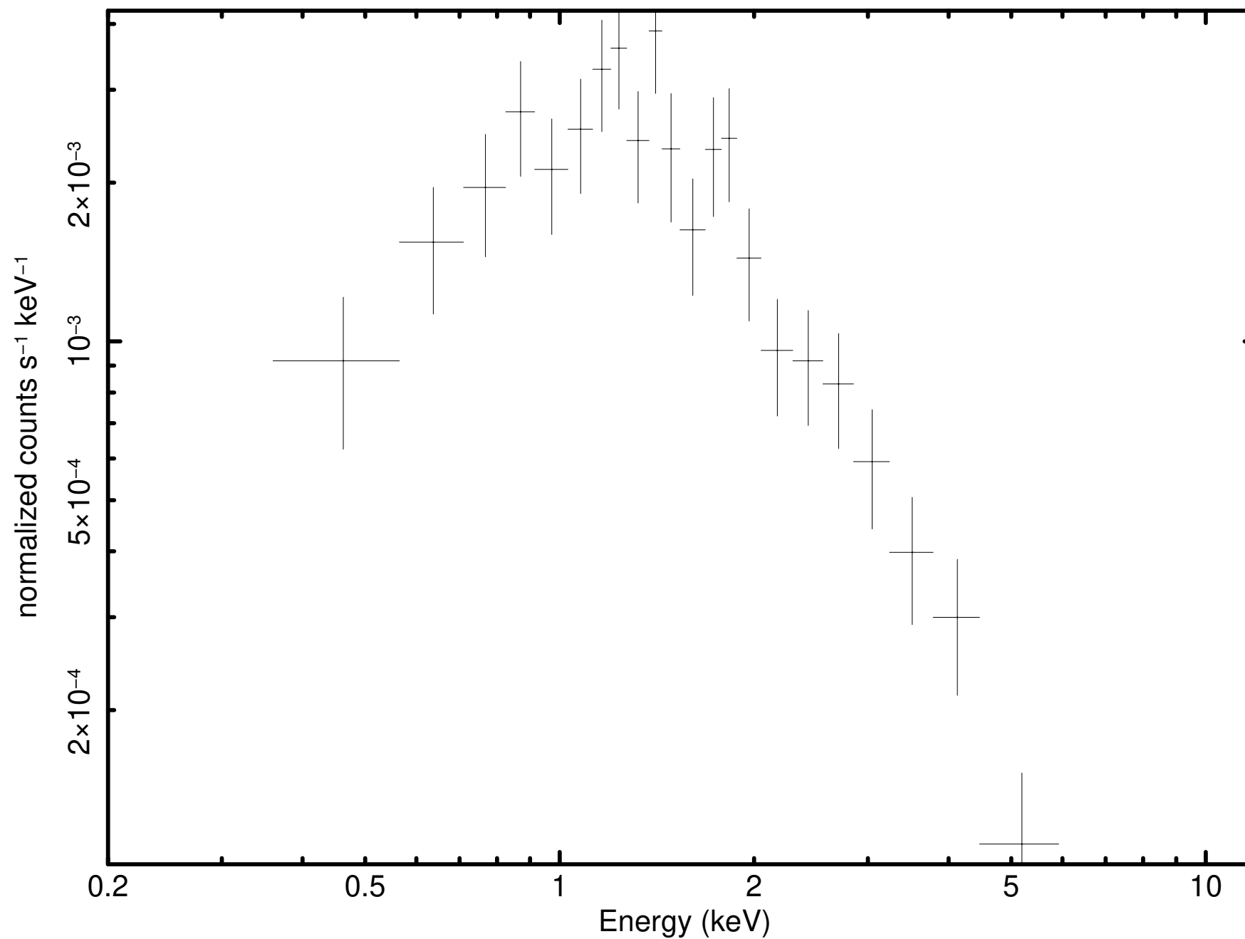
Source 6 minus background (P0931790101M1S001SRSPEC0006)
