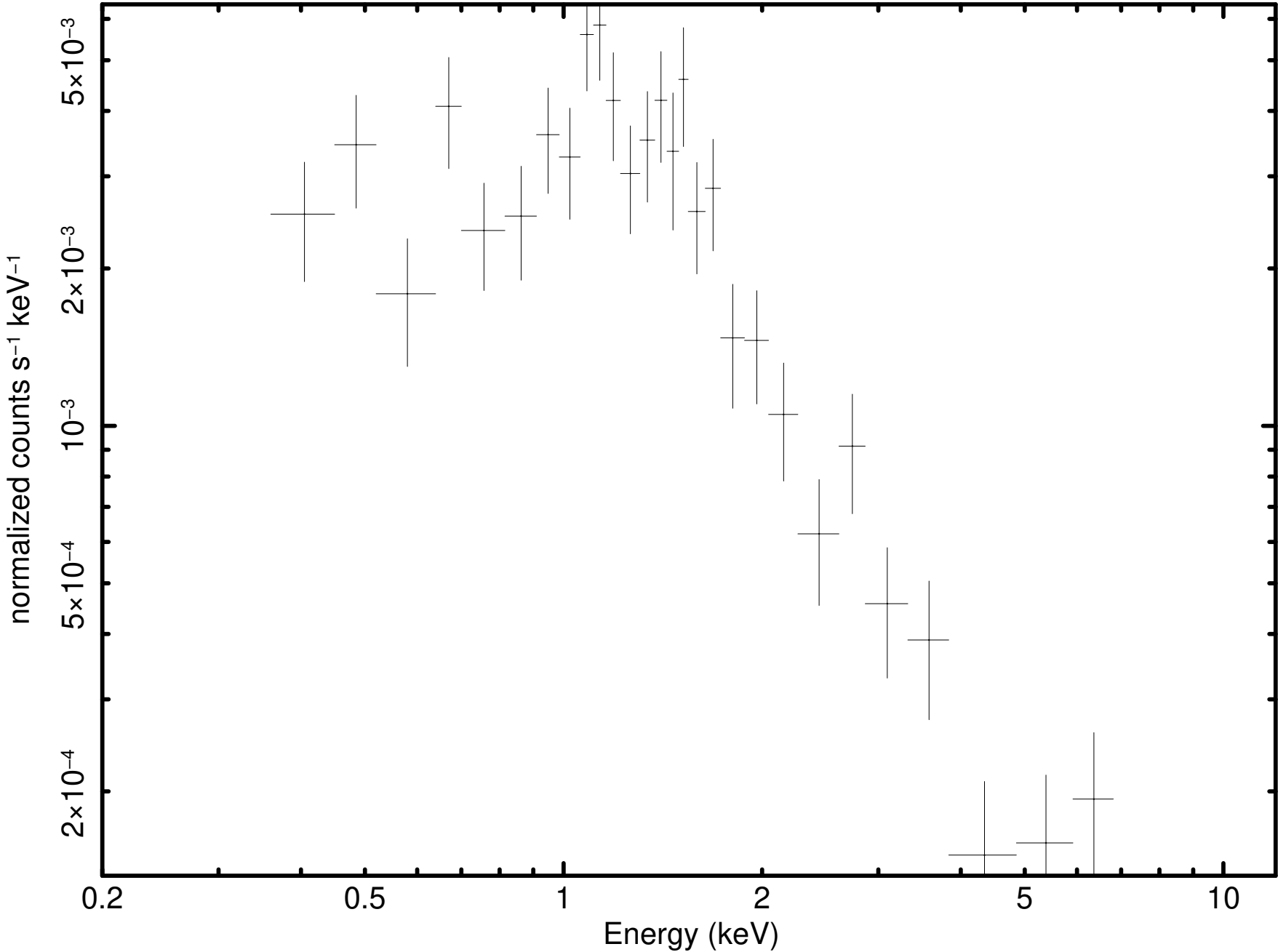
Source 7 minus background (P0931790101M1S001SRSPEC0007)
