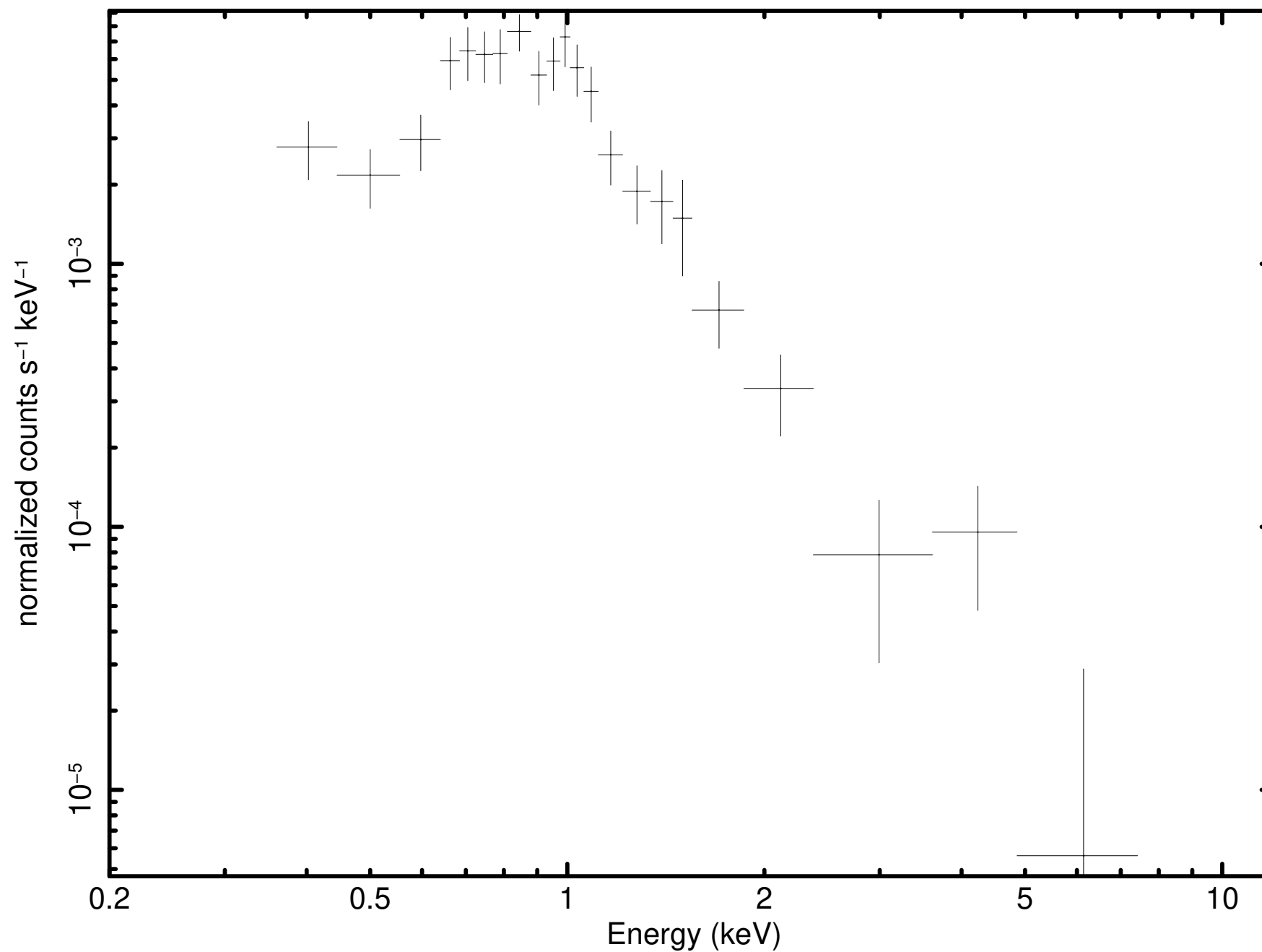
Source 8 minus background (P0931790101M1S001SRSPEC0008)
