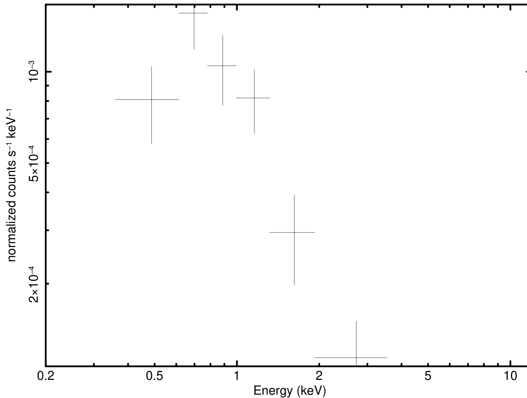
Source 11 minus background (P0931790101M1S001SRSPEC000B)
