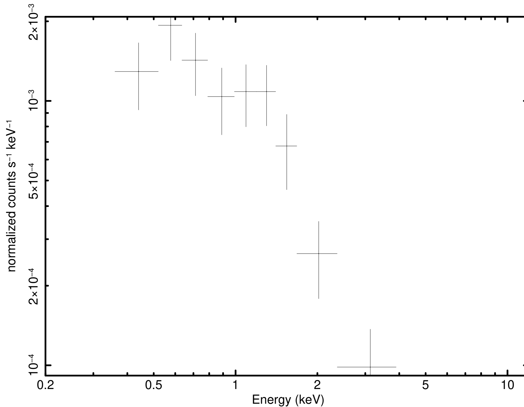
Source 18 minus background (P0931790101M1S001SRSPEC0012)
