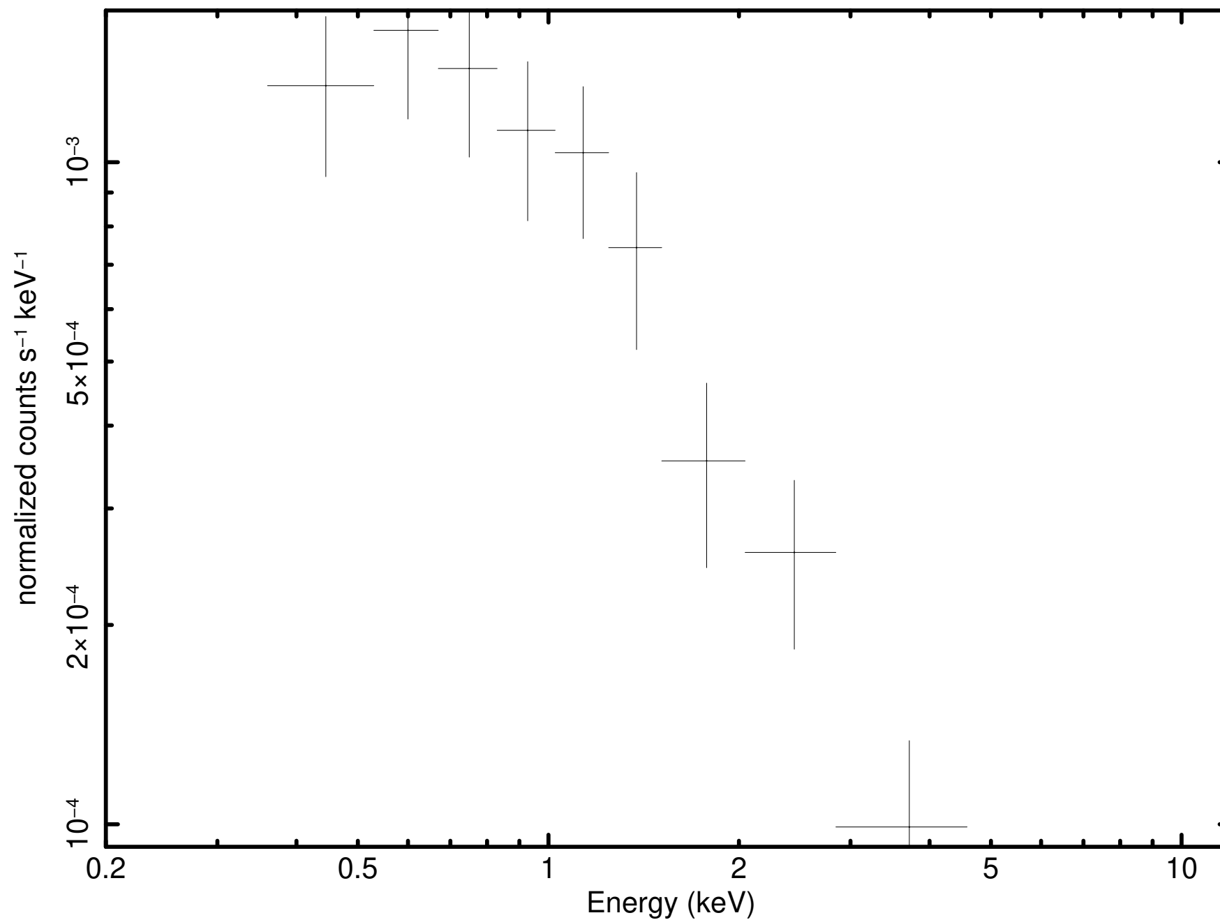
Source 19 minus background (P0931790101M1S001SRSPEC0013)
