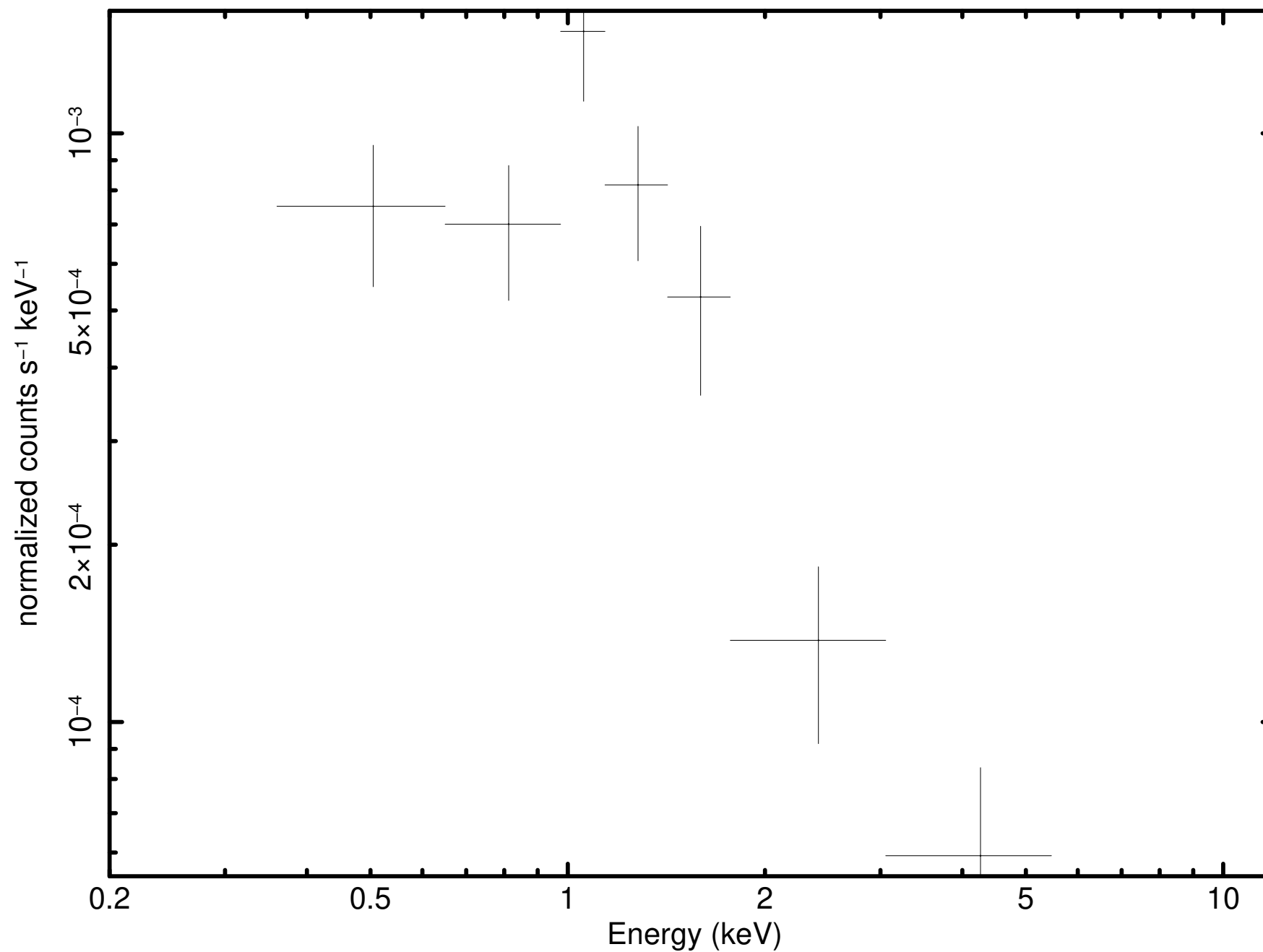
Source 21 minus background (P0931790101M1S001SRSPEC0015)
