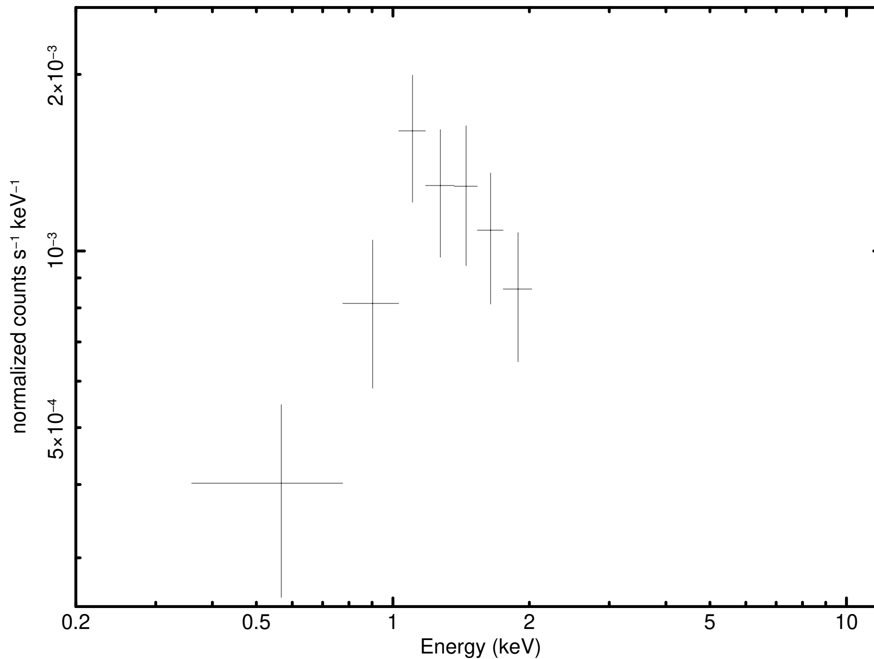
Source 22 minus background (P0931790101M1S001SRSPEC0016)
