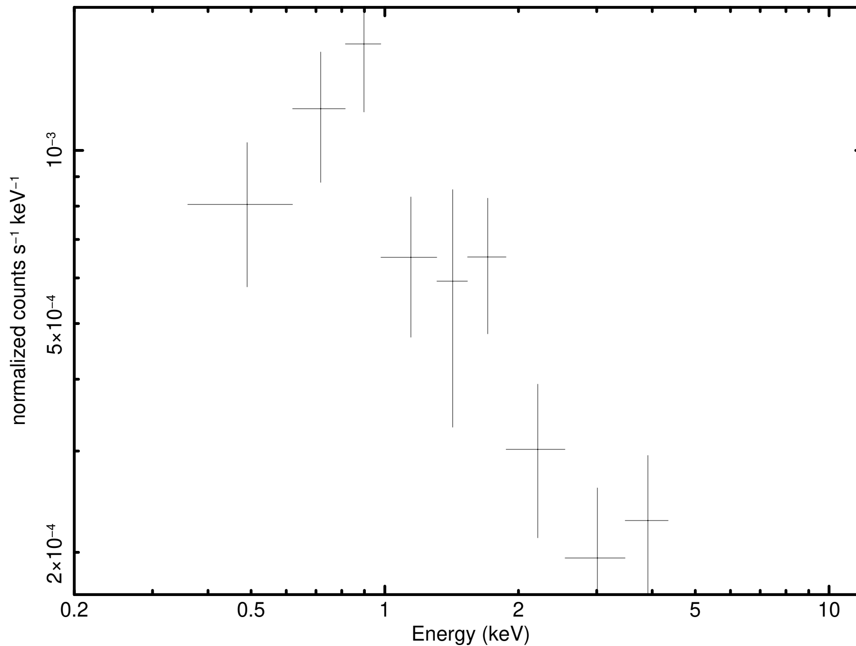
Source 23 minus background (P0931790101M1S001SRSPEC0017)
