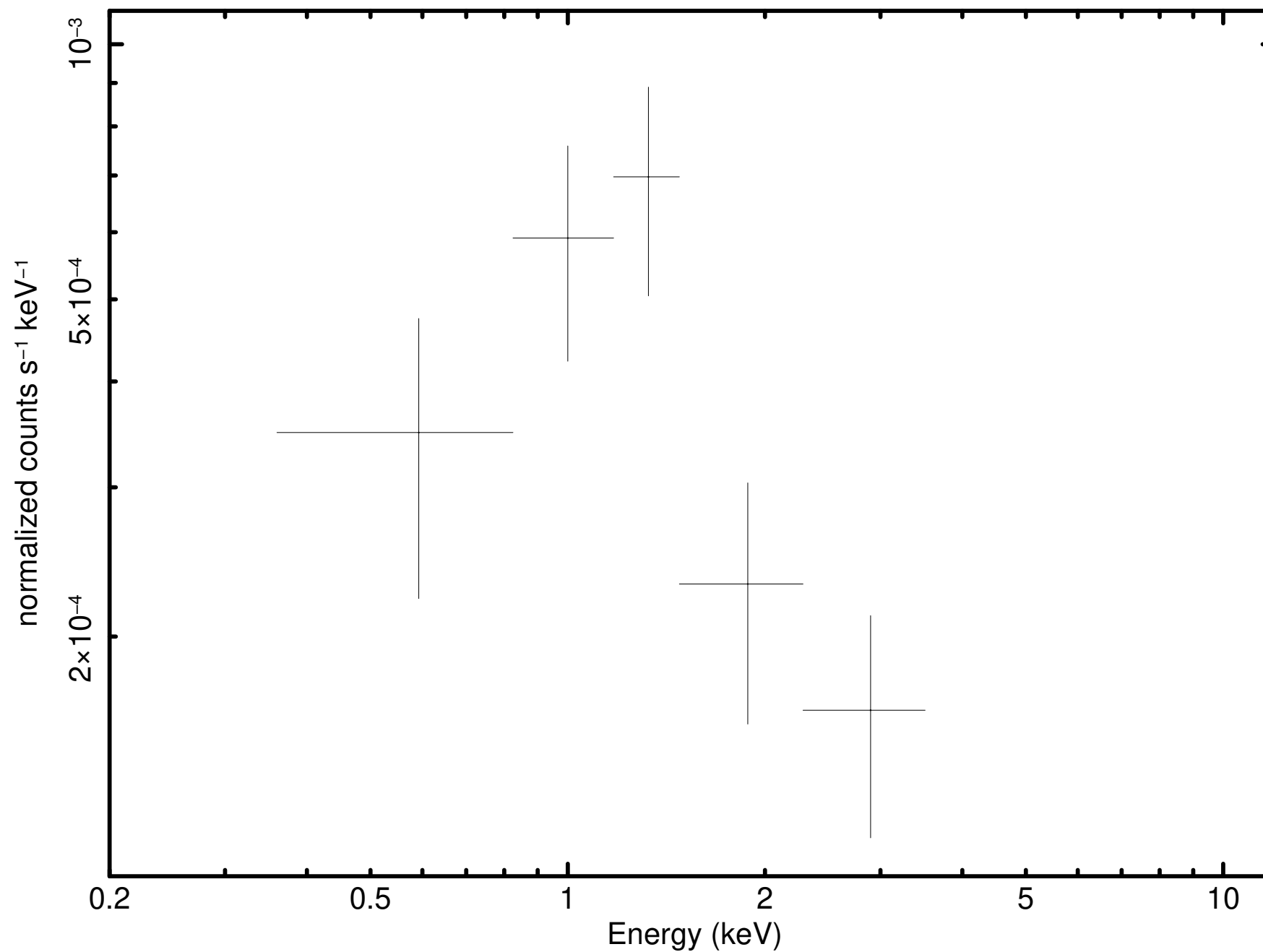
Source 24 minus background (P0931790101M1S001SRSPEC0018)
