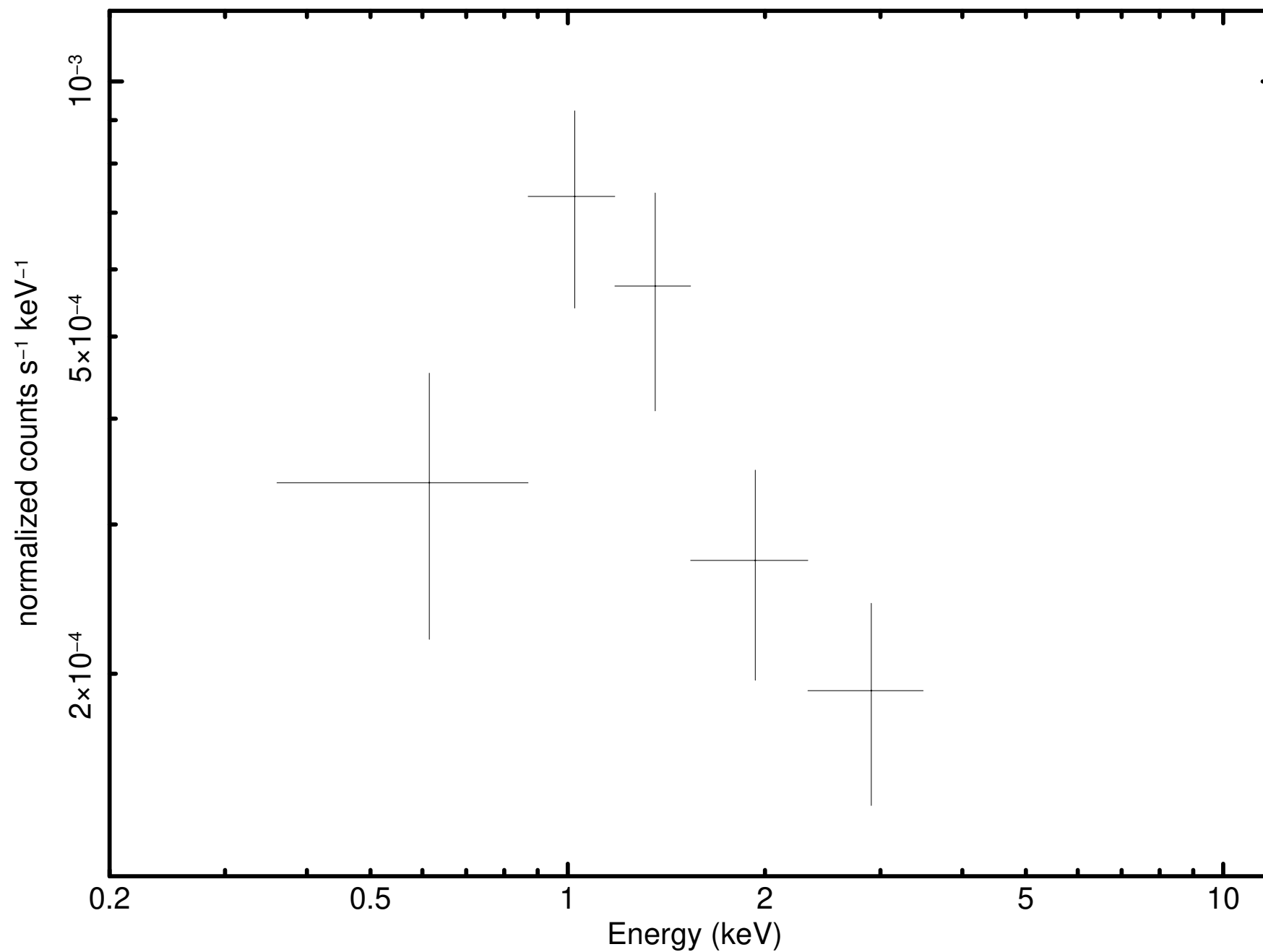
Source 27 minus background (P0931790101M1S001SRSPEC001B)
