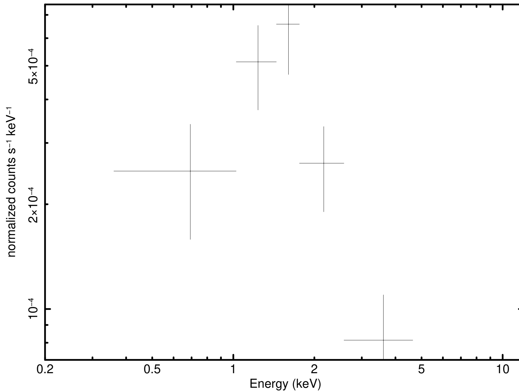
Source 28 minus background (P0931790101M1S001SRSPEC001C)
