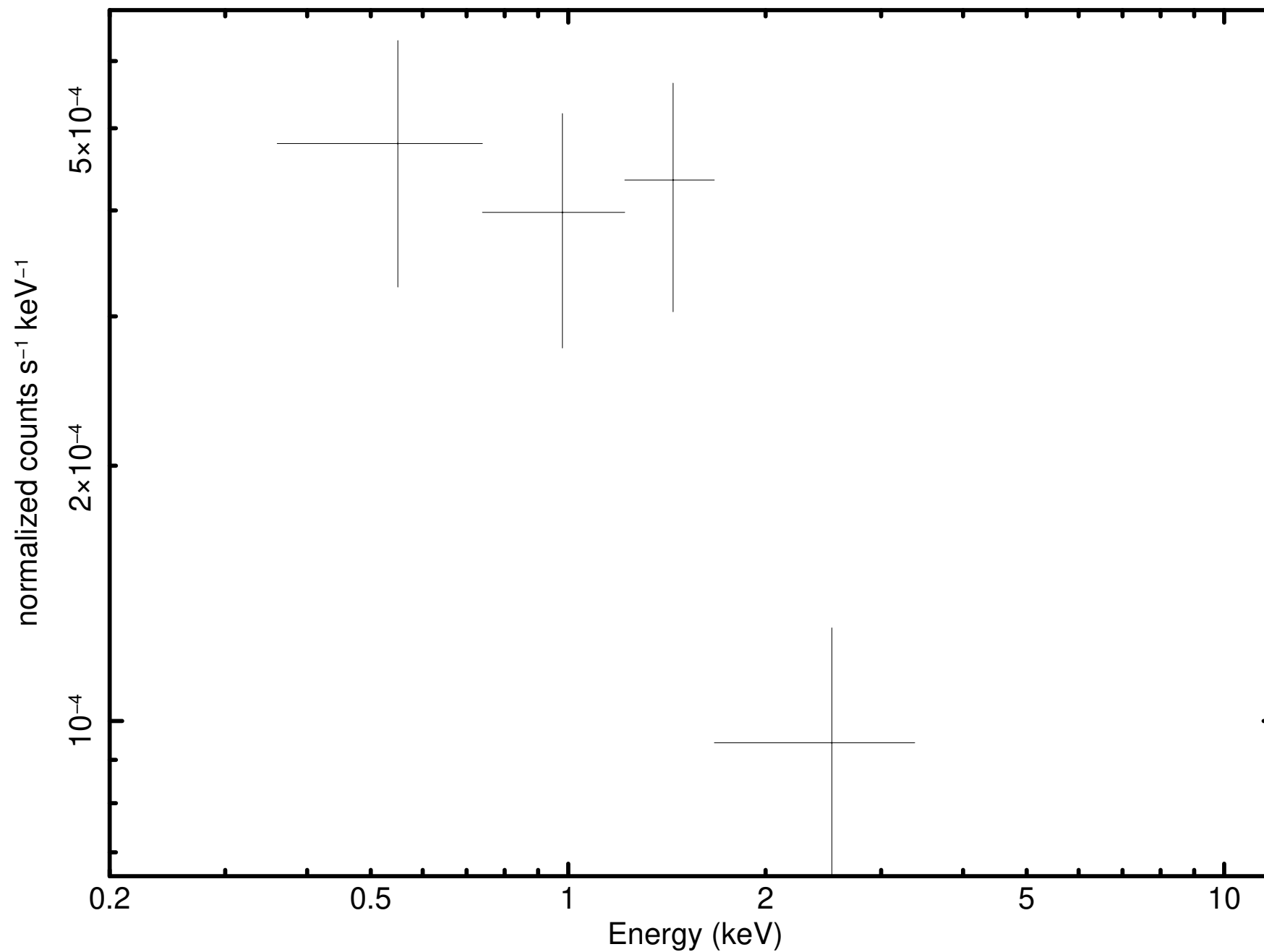
Source 30 minus background (P0931790101M1S001SRSPEC001E)
