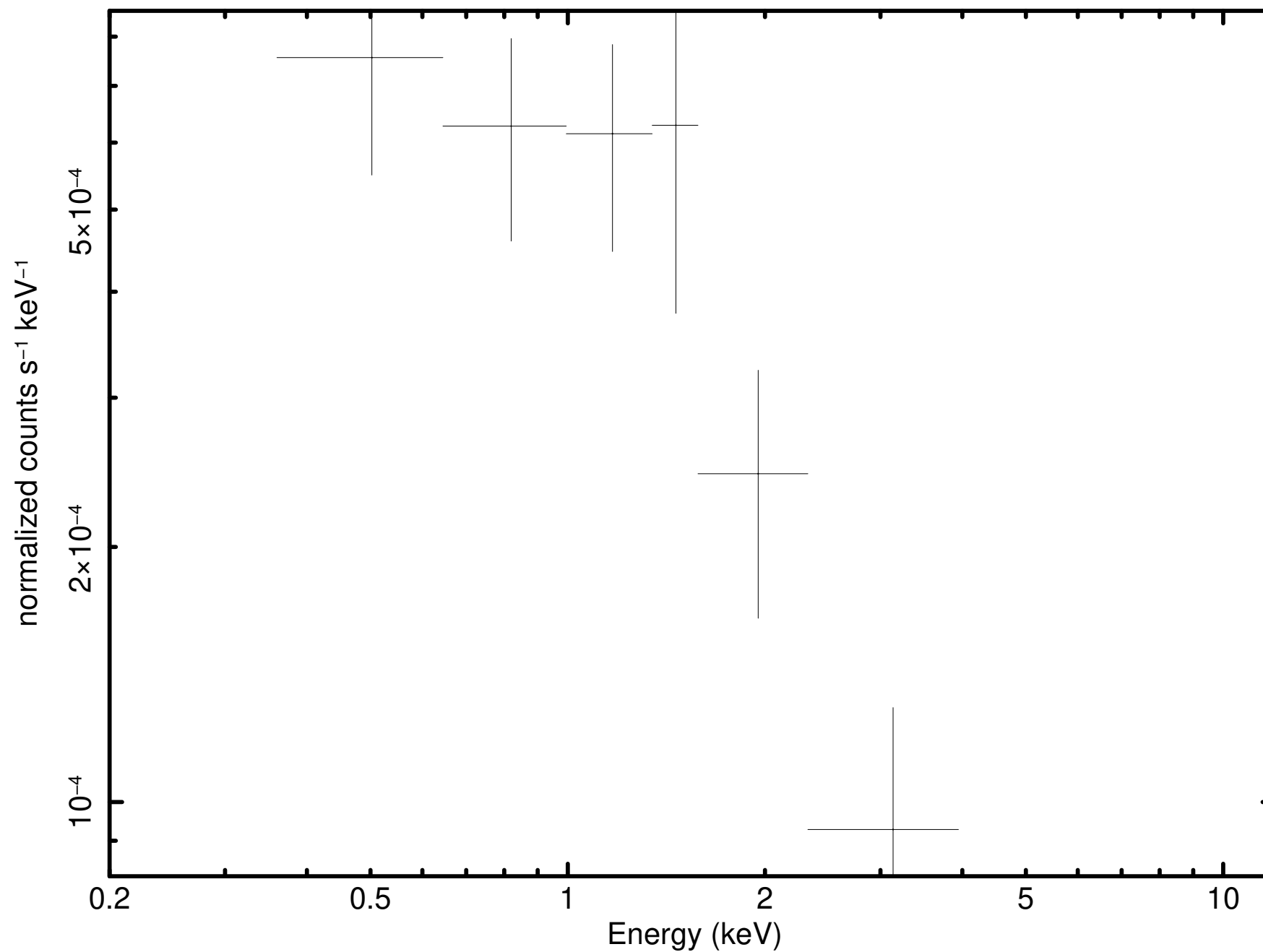
Source 31 minus background (P0931790101M1S001SRSPEC001F)
