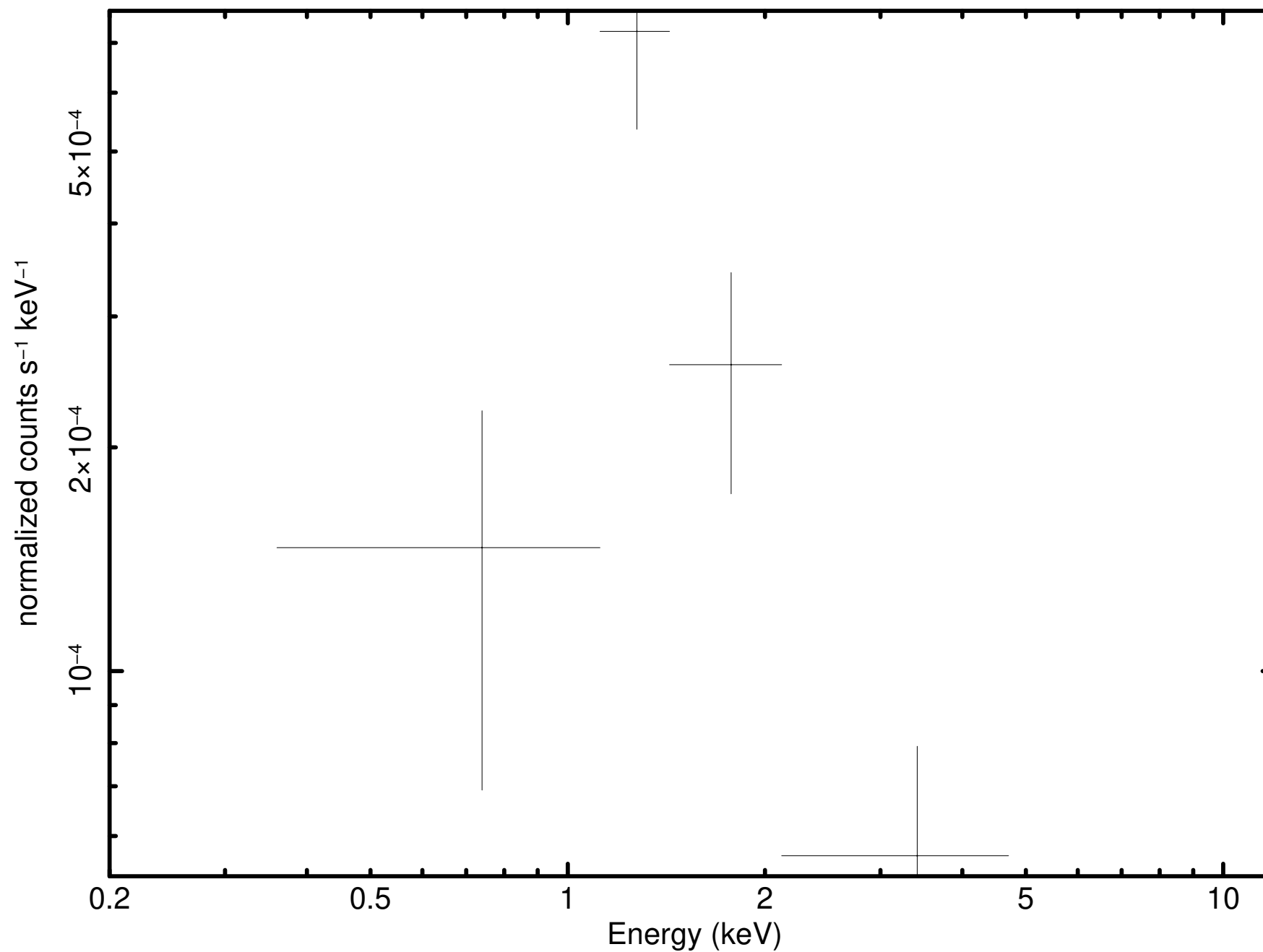
Source 41 minus background (P0931790101M1S001SRSPEC0029)
