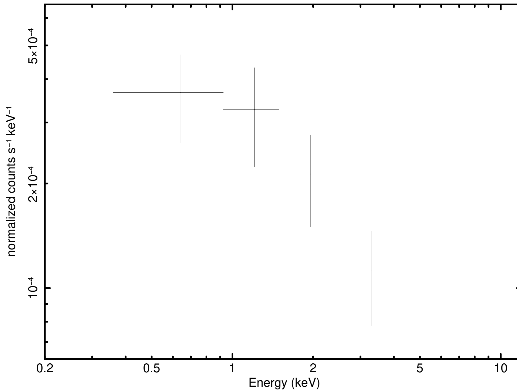
Source 45 minus background (P0931790101M1S001SRSPEC002D)
