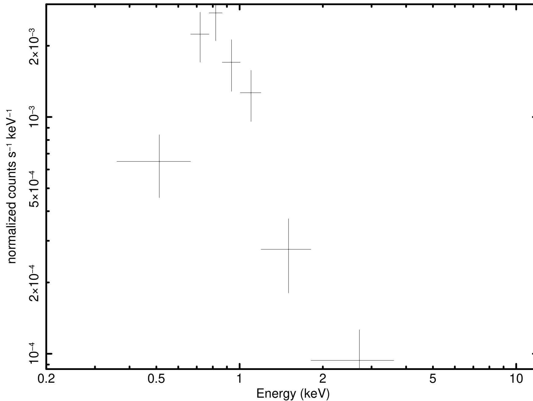
Source 109 minus background (P0931790101M1S001SRSPEC006D)
