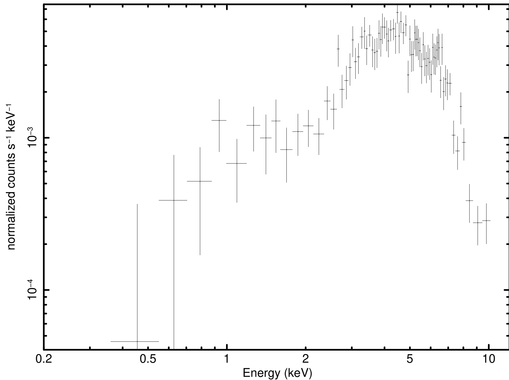
Source 1 minus background (P0931790101M2S002SRSPEC0001)
