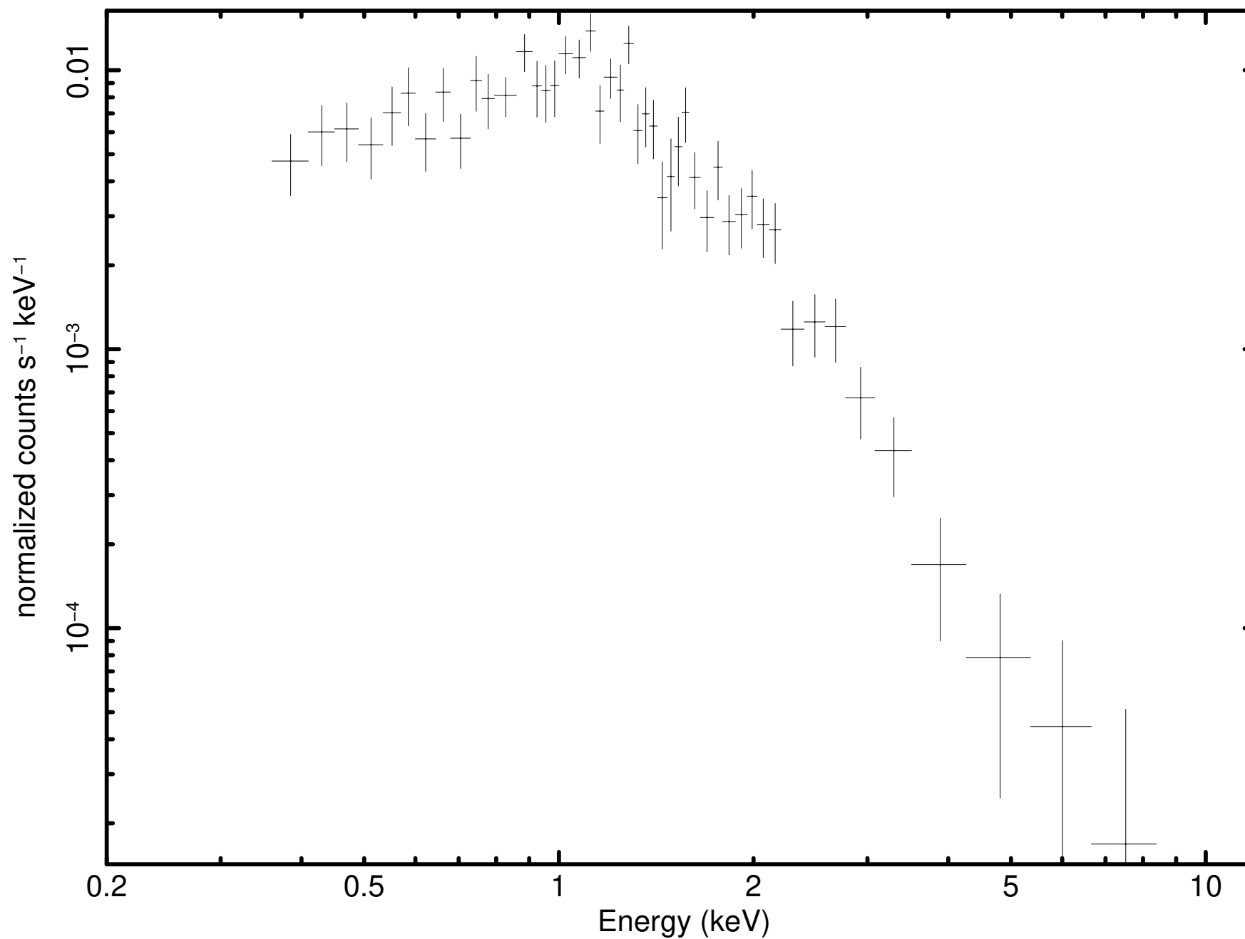
Source 3 minus background (P0931790101M2S002SRSPEC0003)
