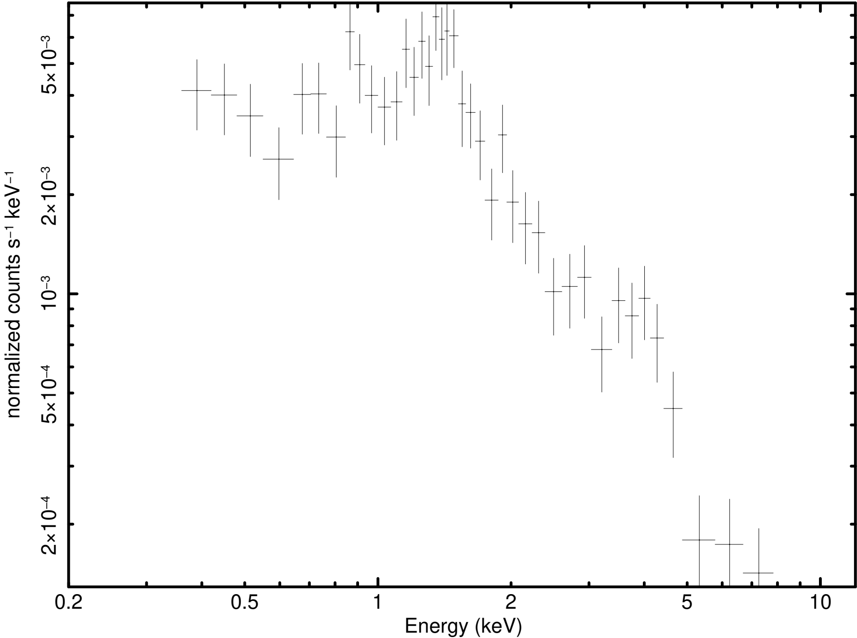
Source 4 minus background (P0931790101M2S002SRSPEC0004)
