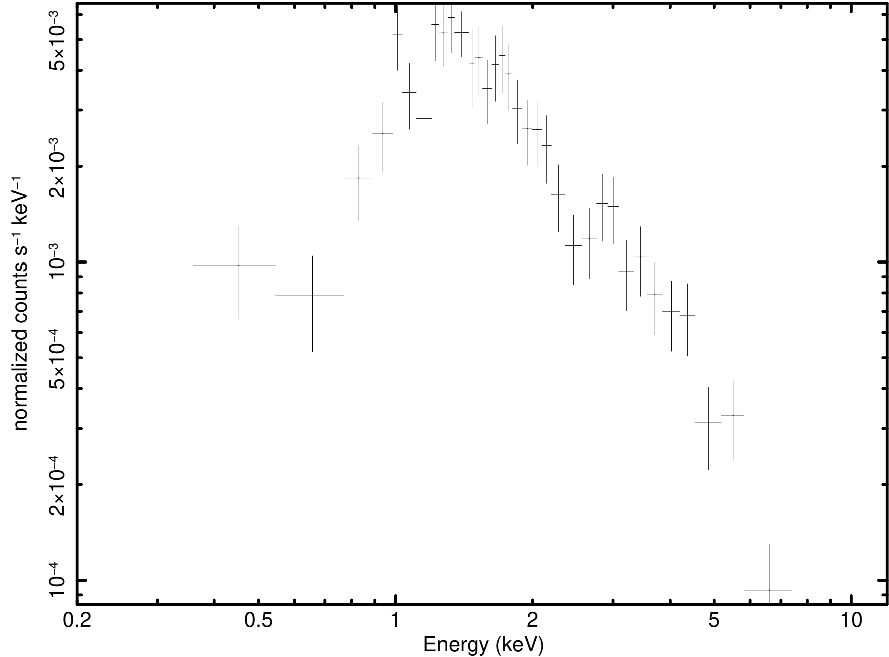
Source 5 minus background (P0931790101M2S002SRSPEC0005)
