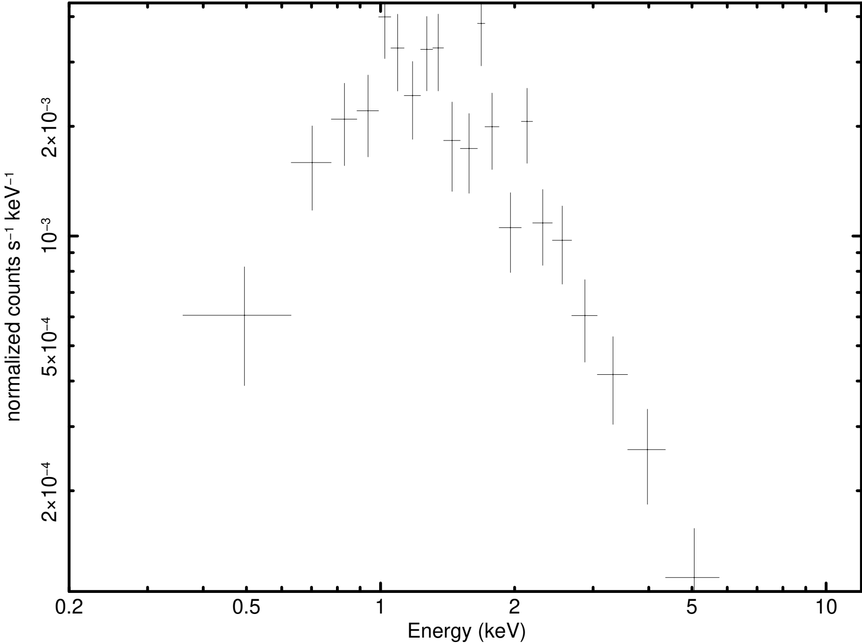
Source 6 minus background (P0931790101M2S002SRSPEC0006)
