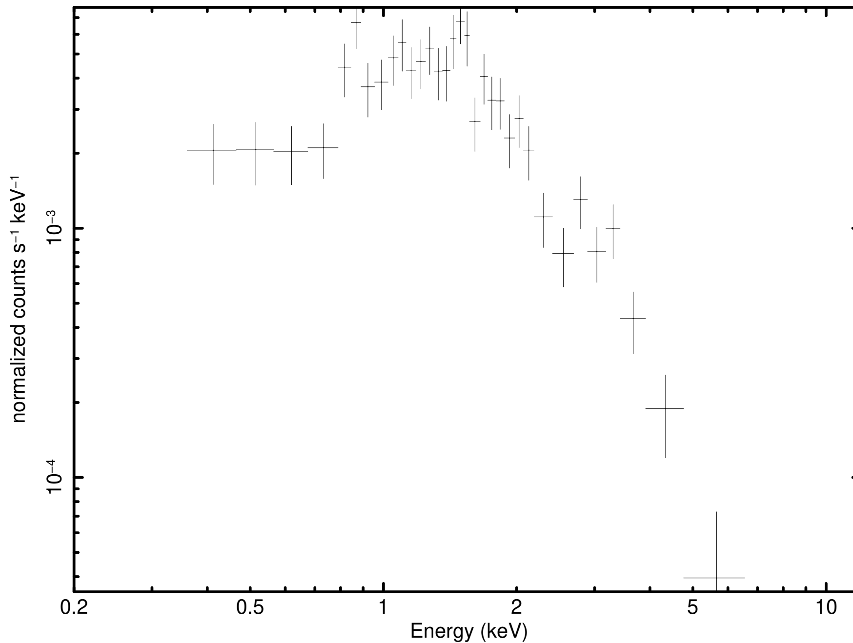
Source 9 minus background (P0931790101M2S002SRSPEC0009)
