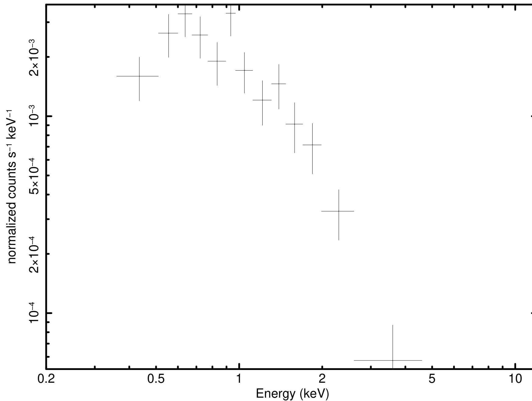
Source 10 minus background (P0931790101M2S002SRSPEC000A)
