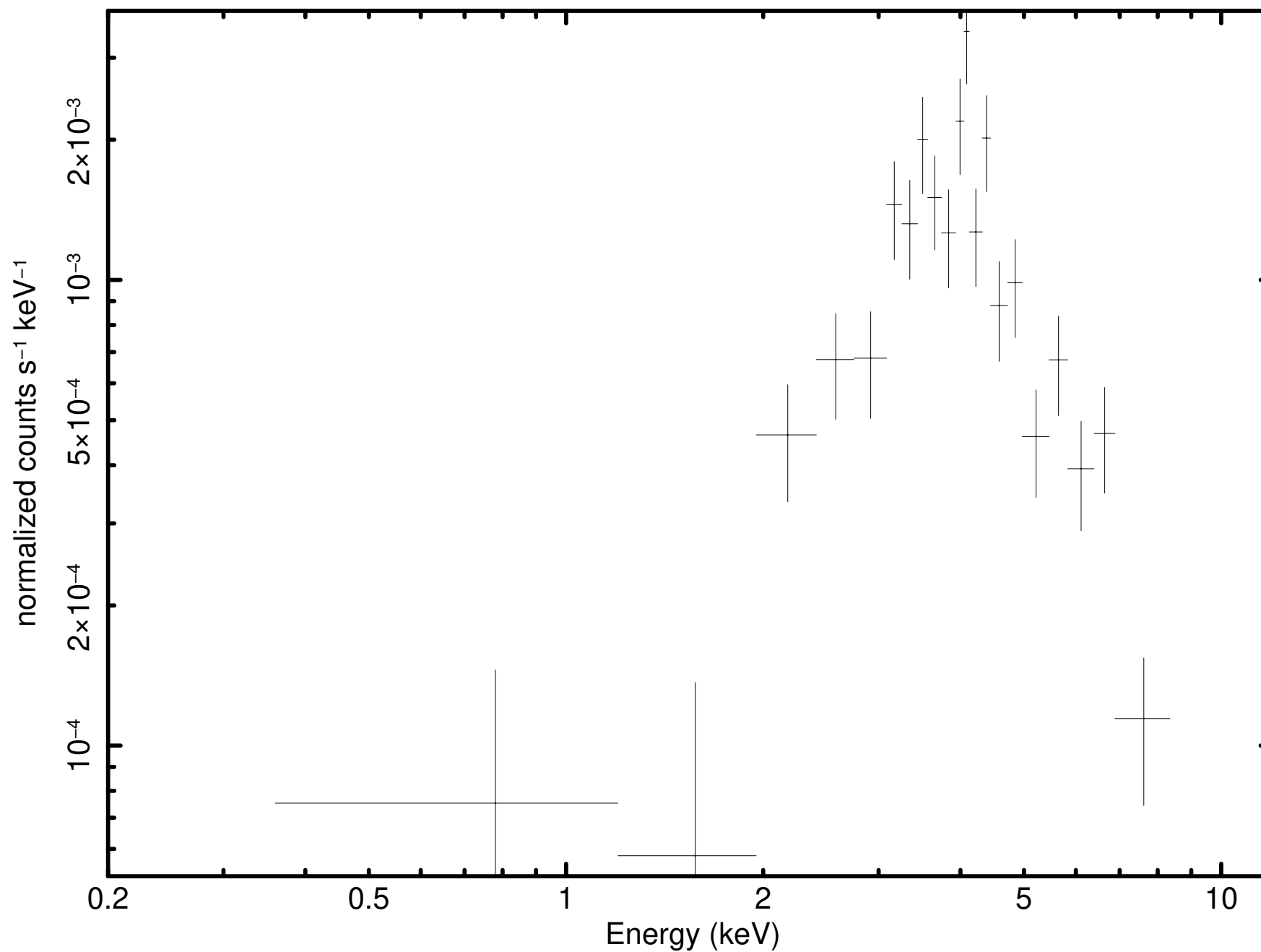
Source 12 minus background (P0931790101M2S002SRSPEC000C)
