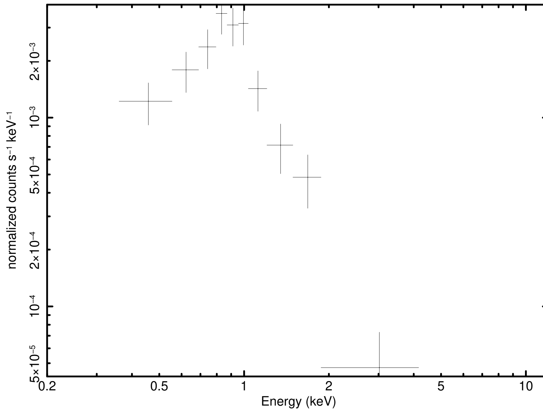
Source 14 minus background (P0931790101M2S002SRSPEC000E)
