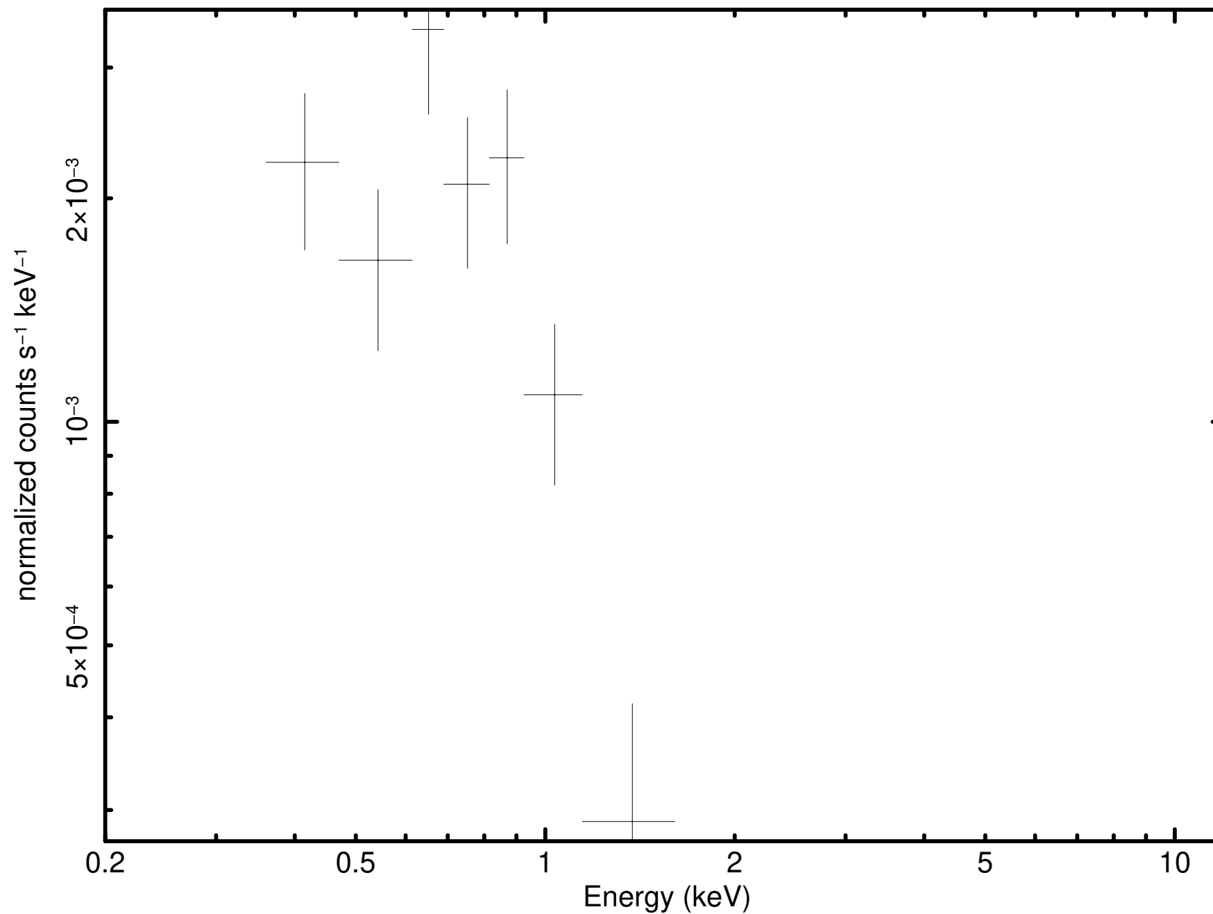
Source 15 minus background (P0931790101M2S002SRSPEC000F)
