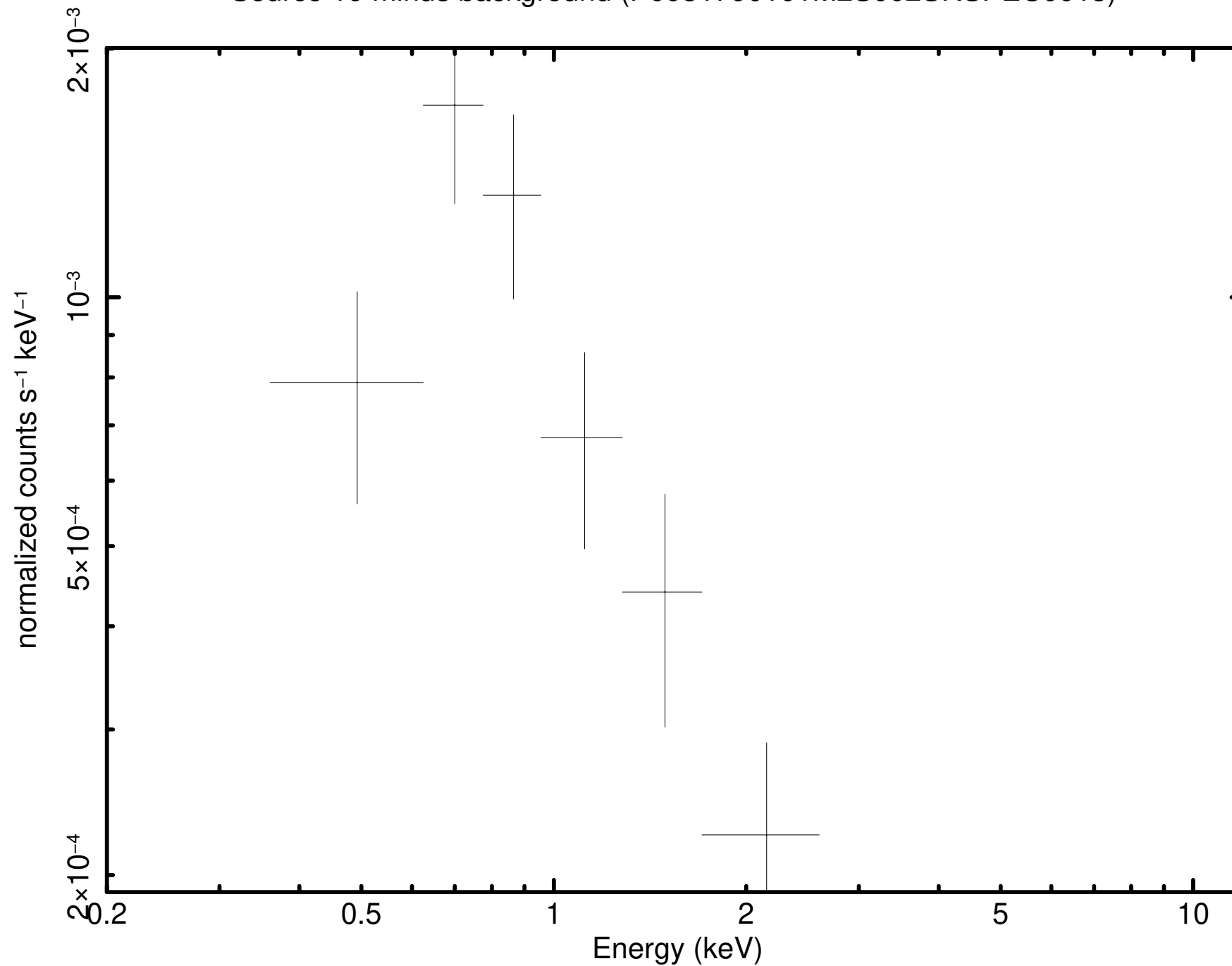
Source 19 minus background (P0931790101M2S002SRSPEC0013)
