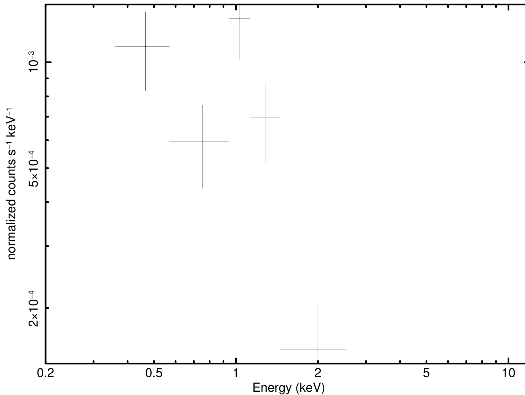
Source 20 minus background (P0931790101M2S002SRSPEC0014)
