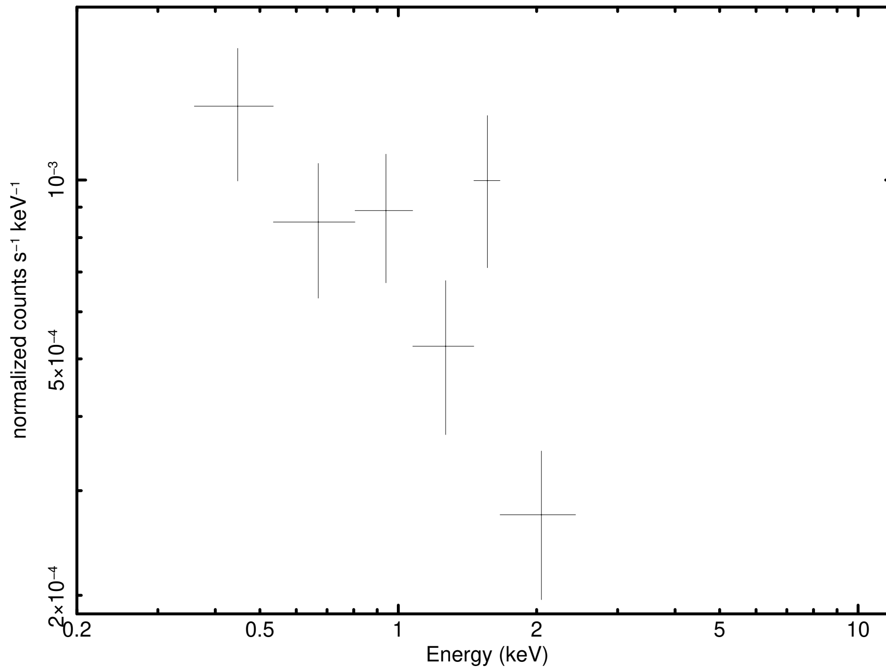
Source 21 minus background (P0931790101M2S002SRSPEC0015)
