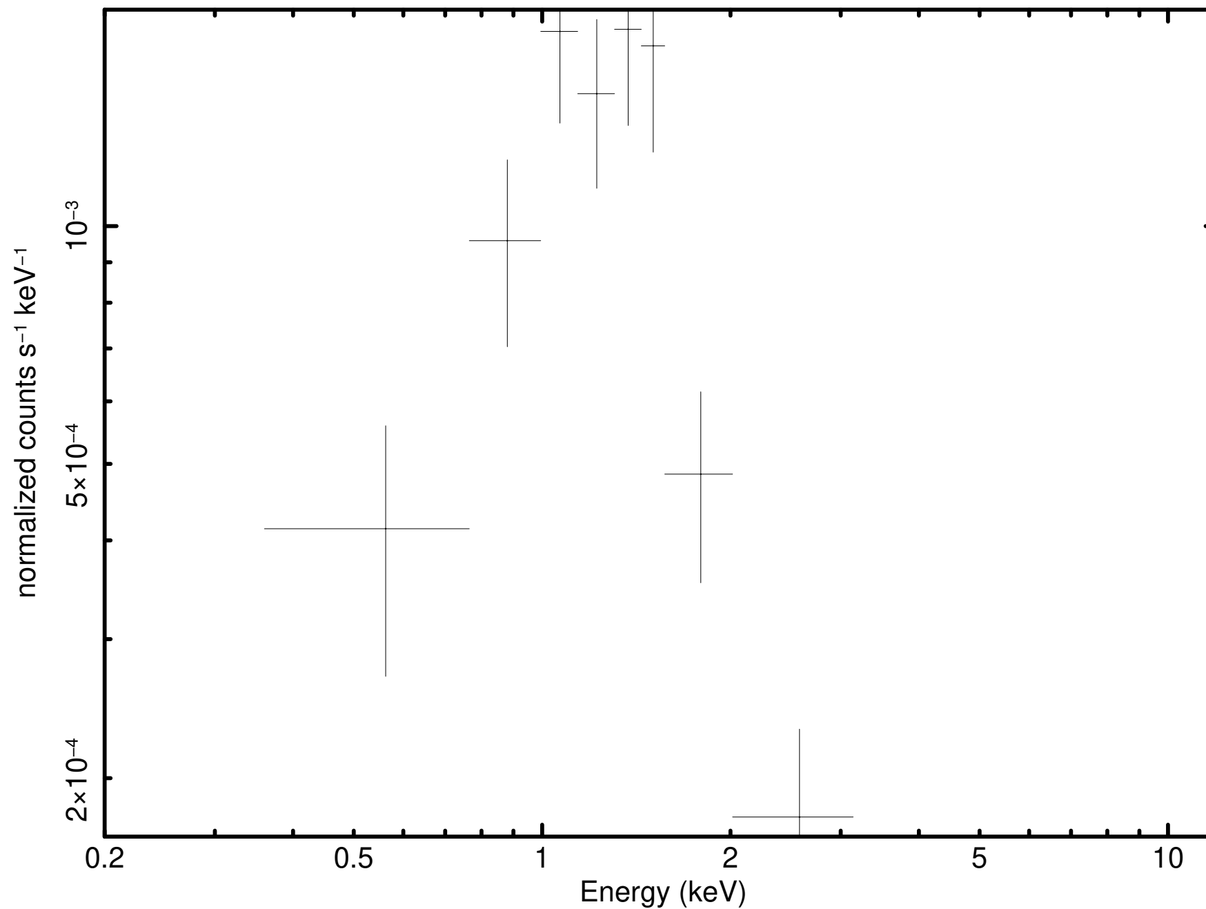
Source 22 minus background (P0931790101M2S002SRSPEC0016)
