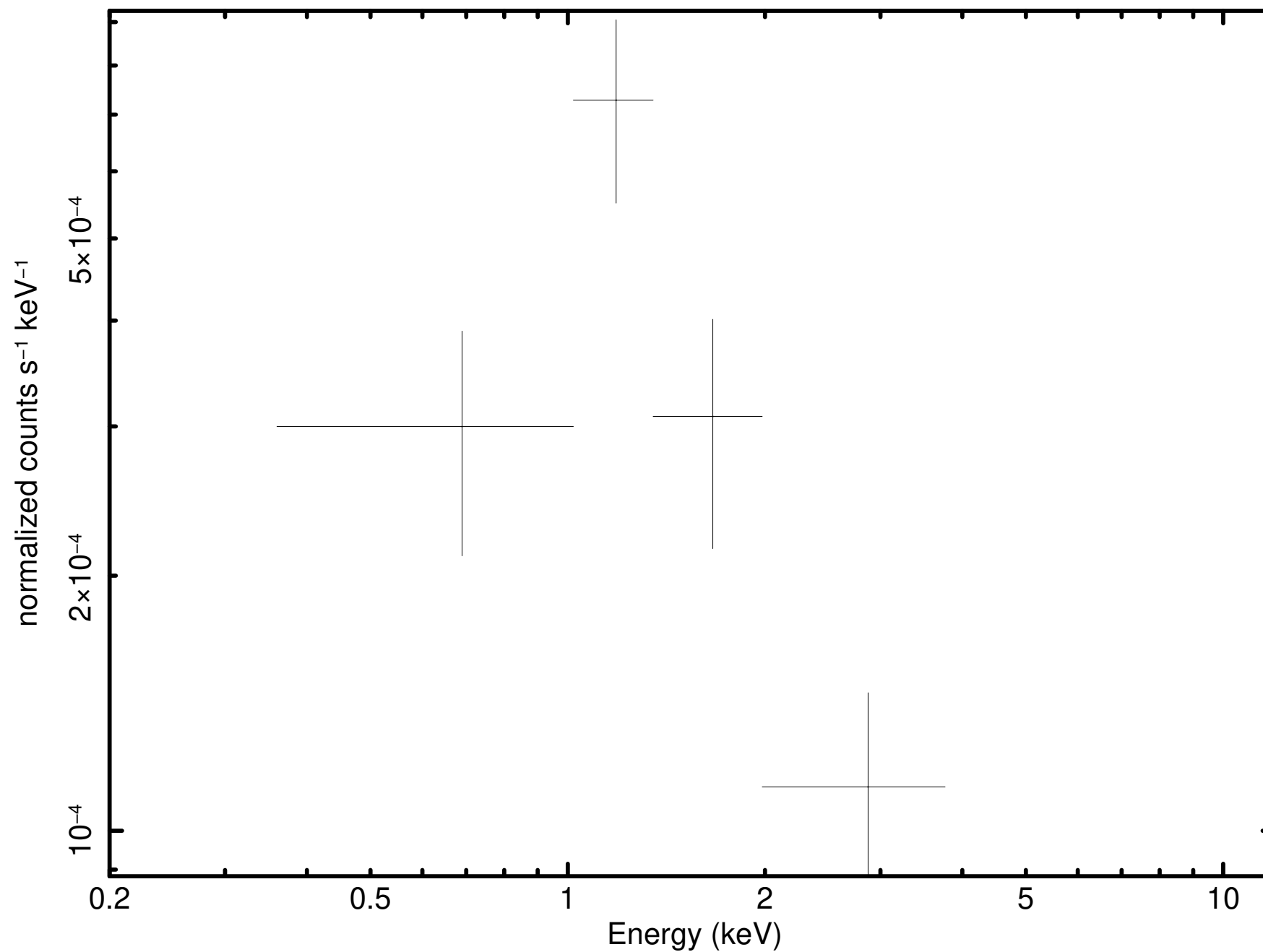
Source 26 minus background (P0931790101M2S002SRSPEC001A)
